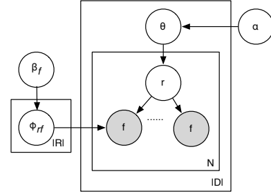
Figure 1: Rel-LDA model. Shaded circles are observations, and unshaded ones are hidden variables. A document consists of N tuples. Each tuple has a set of features. Each feature of a tuple is generated independently from a hidden relation variable r .
