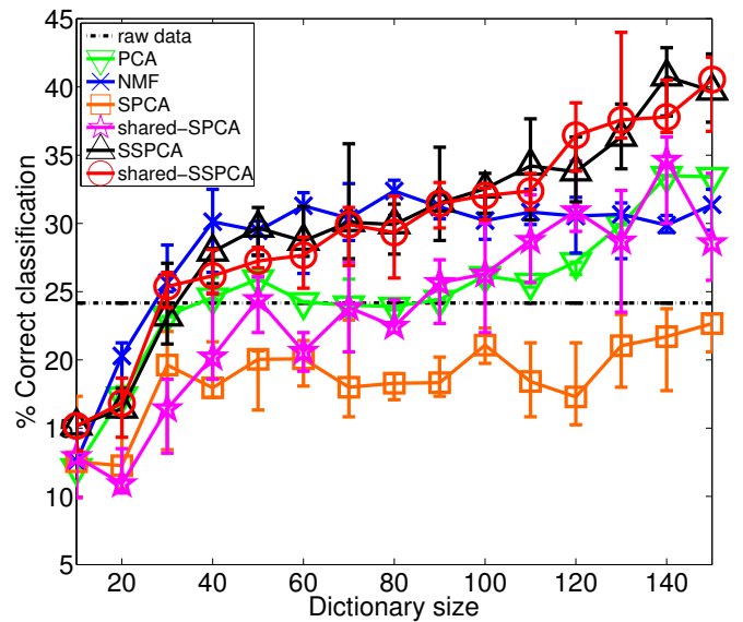
Figure 4: Classification accuracy versus dictionary size: each dimensionality reduction technique is used with k-NN to classify occluded faces. SSPCA shows better robustness to occlusions. The points, lower and upper error bars on the curves respectively represent the median, first and third quartile, based on 10 runs.
