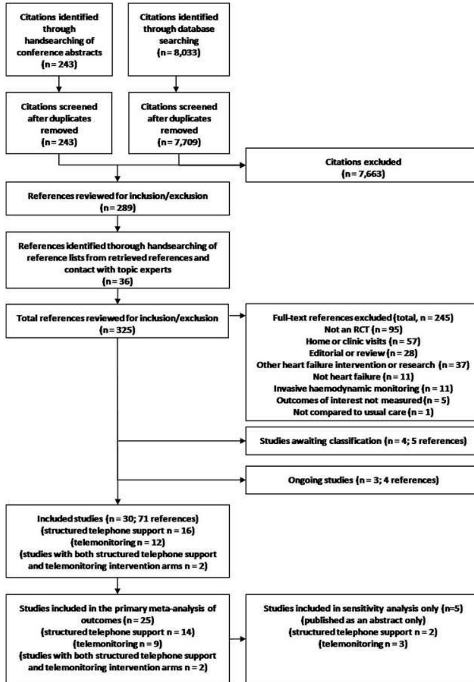
Figure 3. Study flowchart.
