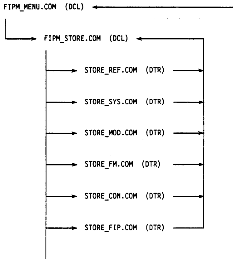
FIGURE 33. PROGRAM FLOW FOR STORING FIPM DATA
