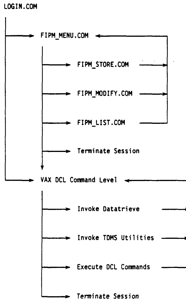
FIGURE 31. TOP-LEVEL FIPM SOFTWARE FLOWS
