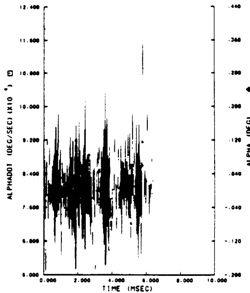
FIGURE 61. HIGH-FREQUENCY CAGE INSTABILITY WITH 2X FREQUENCY SUPERIMPOSED. CALCULATED BY BASDAP (Reference 8)
