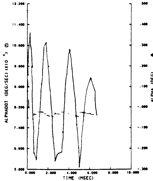
FIGURE 60. IMPACT OF CAGE AND BALLS AT APPROXIMATELY 450 HZ. CALCULATED BY BASDAP FOR A MARGINALLY STABLE CASE (Reference 8)
