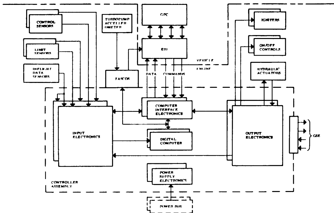
FIGURE 65. SSME CONTROLLER ORGANIZATION
