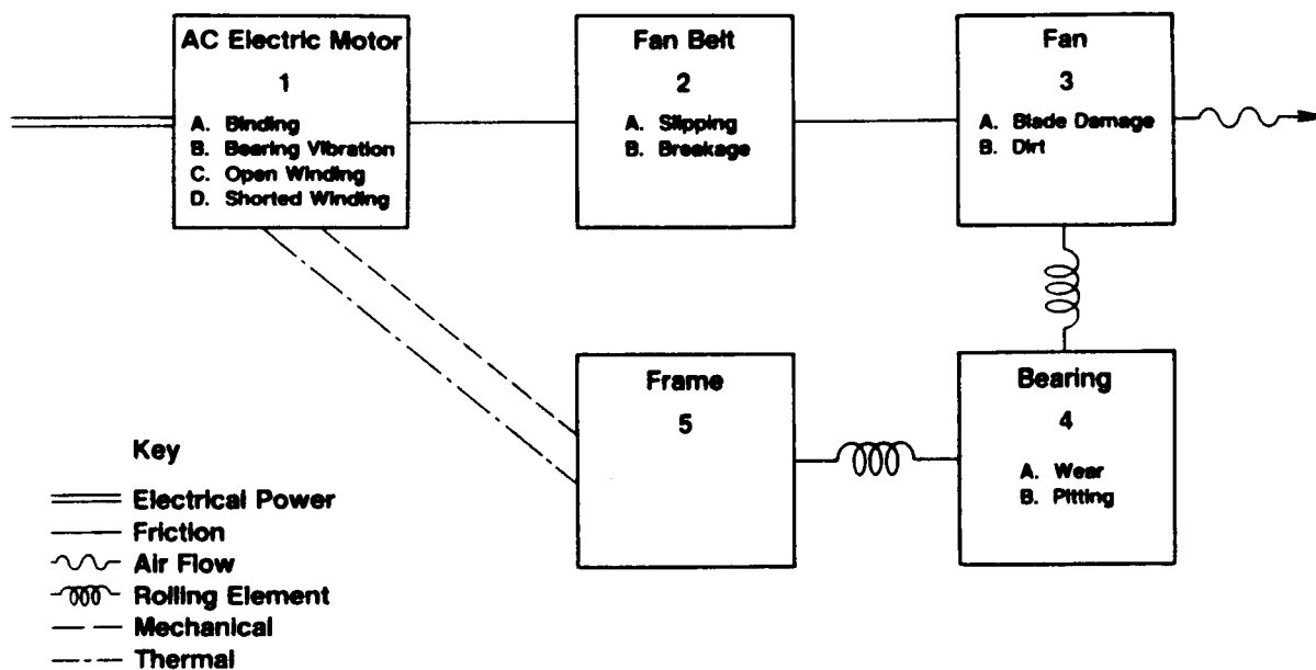
FIGURE 16. ADDITION OF FAILURE MODES TO EXHAUST FAN FIPM
