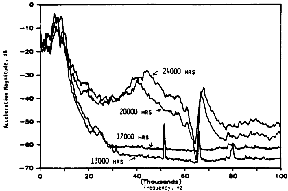
FIGURE 64. VIBRATION SPECTRAL DATA FOR THE BEARING SERVICE LIFE IN A POWER PLANT AXIAL-FLOW FAN. (REFERENCE 9)
