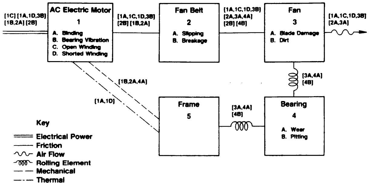
FIGURE 18. FAILURE INFORMATION GROUPED BY SIGNAL TYPE FOR THE EXHAUST FAN FIPM
