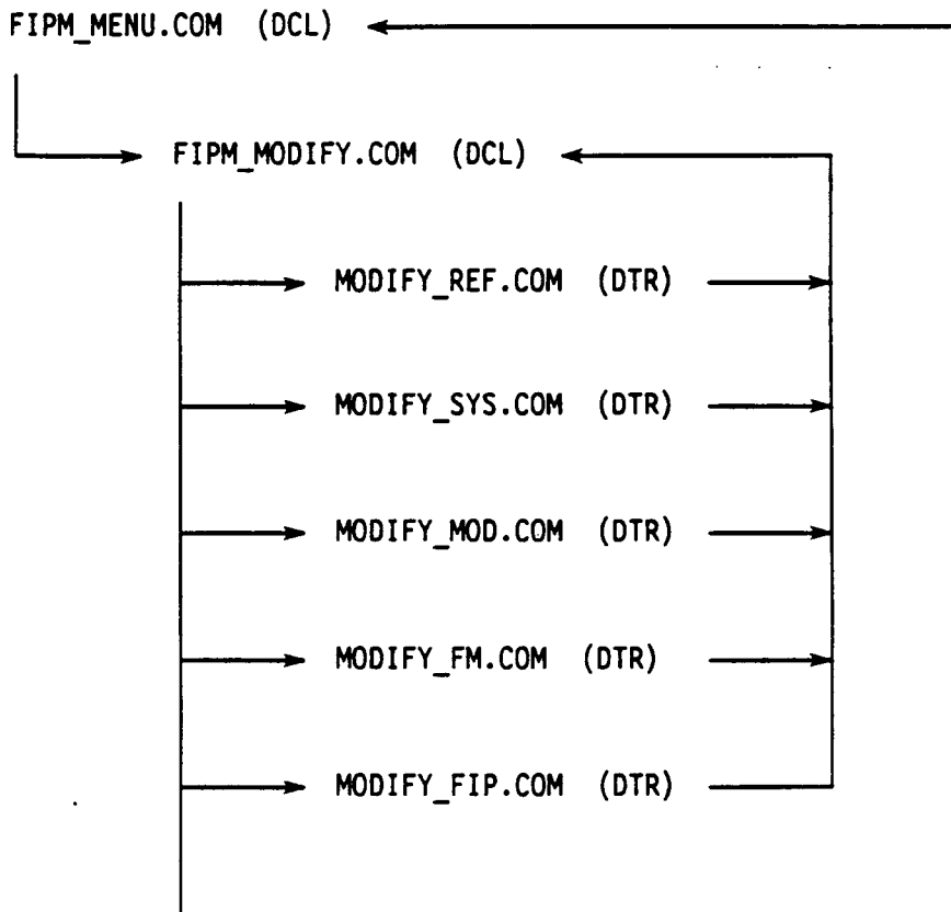
FIGURE 35. PROGRAM FLOW FOR MODIFYING FIPM DATA
