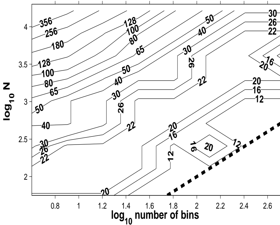
Figure 5: Simulation study, based on the false positive rate of 0.05, to determine \text{ncp\_prior} = -\log(\gamma) for binned data. Contours of this parameter are shown as a function of the number of bins and number of data points (logarithmic x- and y- axes, respectively). The heavy dashed line indicates the undesirable region where the numbers of bins and data points are equal.
