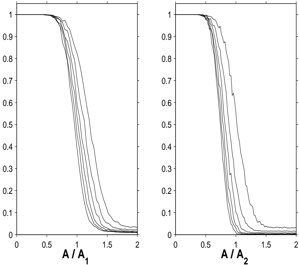
Figure 4: Error in finding a single block vs. simulated block amplitude in units of Arias-Castro et al. 's threshold amplitude. The curves (from right to left) are for N = 32, 64, 128, 256, 1024 and 2048 .
