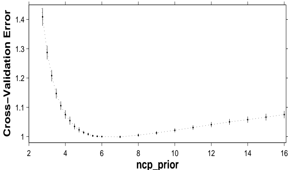
Figure 1: Cross-validation error of BATSE TTE data (averaged over 532 GRBs, 8 random subsamples, and time) for a range of values of -\log \gamma = with 3\sigma error bars.
