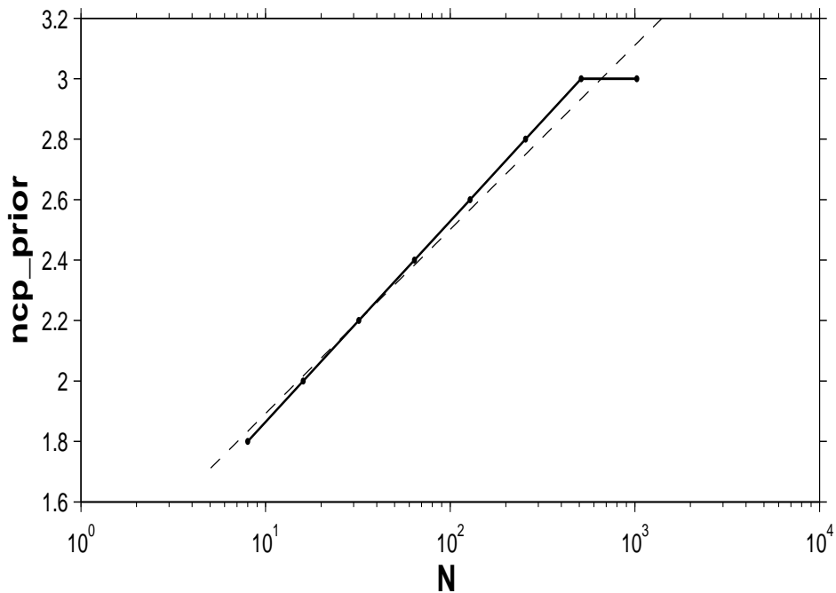
Figure 6: Simulations of point measurements (Gaussian noise with signal-to-noise ratio of 10) to determine \text{ncp\_prior} = -\log(\gamma) . Top: false positive fraction p_0 vs. value of \text{ncp\_prior} with separate curves for the values N = 8, 16, 32, 64, 128, 256, 512 and 1024 (left to right; alternating dots, + and circles). The points at which the rate becomes unacceptable (here .05; dashed line) determines the recommended values of \text{ncp\_prior} shown as a function of N in the bottom panel.
