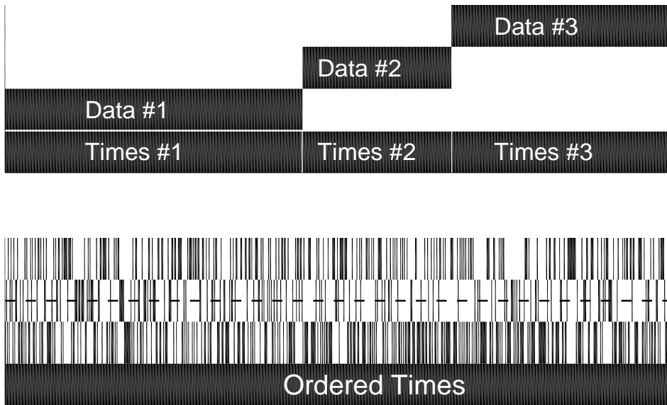
Figure 2: Cartoon depicting an example of how three data series are first concatenated into a matrix (top) and then redistributed by ordering the combined time-tags (bottom). The cost functions for the series can then be computed from the data in horizontal slices ( e.g. dashed line) and combined, allowing the change-points to be at any of the time tags.
