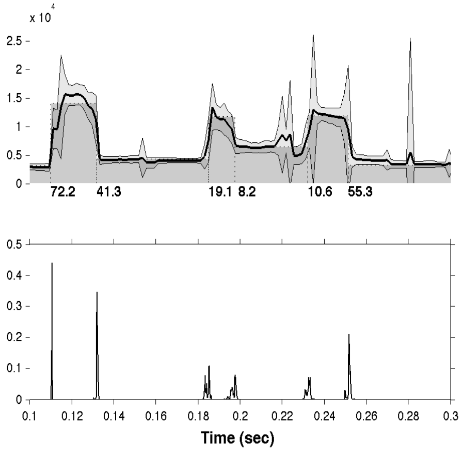
Figure 8: Error analysis for the data in Channel 4 from Fig. 7, zooming in on the time interval with most of the activity. Top: Heavy solid line is bootstrap mean (256 realizations), with thin lines giving the \pm 1\sigma RMS deviations, all superimposed on the BB representation. Bottom: approximate posterior distribution functions for the locations of the change-points, obtained by fixing all of the others.
