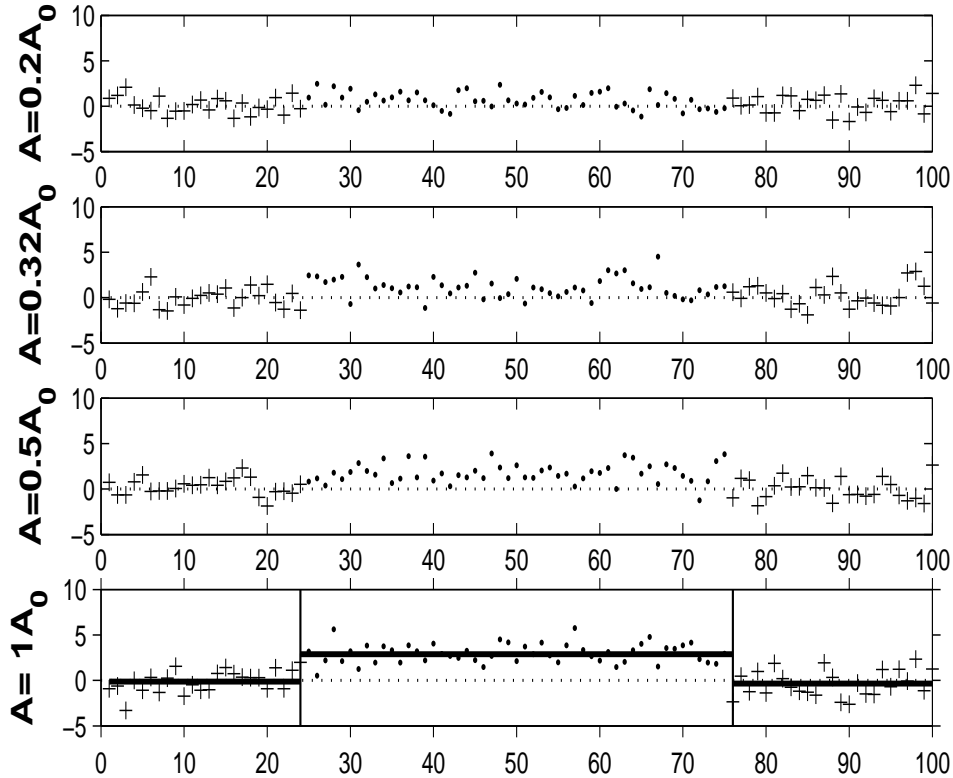
Figure 3: One hundred unit variance normally distributed measurements – zero-mean (+) except for a block of events 25-75 (dots). In the four panels the block amplitudes are 0.2, .32, .5, and 1.0 in units of the Arias-Castro et al. threshold \sqrt{2 \log N} . Thick lines show the blocks, where detected, with thin vertical lines at the change-points.
