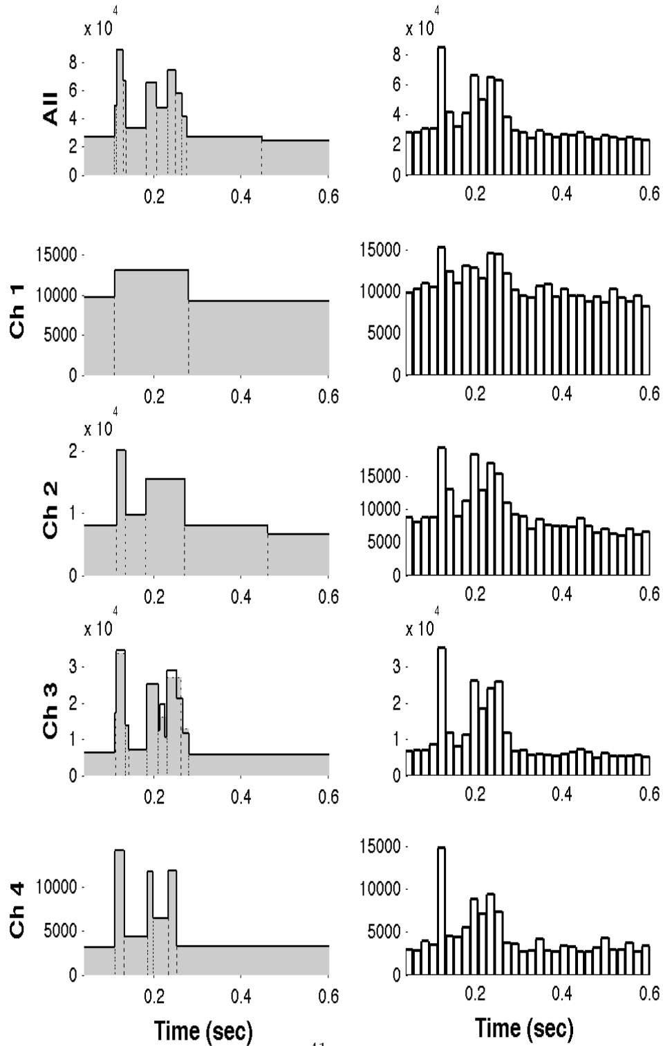
Figure 7: BATSE TTE data for Trigger 0551. Top panels: all photons. Other panels: photons in the four BATSE energy channels. Left column shows Bayesian Block representations: default ncp_prior = solid lines; iterated ncp_prior = shaded/dashed lines. Right column: ordinary evenly spaced binned histograms.
