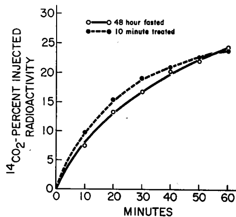
FIG. 4. PALMITATE-1- ^{14} C OXIDATION TO ^{14} CO 2 IN VIVO IN THE REVERSAL OF KETOSIS. Experimental details are outlined in the text. Fasted and treated curves were obtained in the same animal. Acetoacetate concentration in the blood immediately before the injection of insulin and glucose was 11.6 mg per 100 ml. Eight minutes after insulin acetoacetate was 4.6 mg per 100 ml, and at the end of the experiment the level was 1.6 mg per 100 ml. Palmitate-1- ^{14} C in the treated curve was administered 10 minutes after insulin and glucose.
