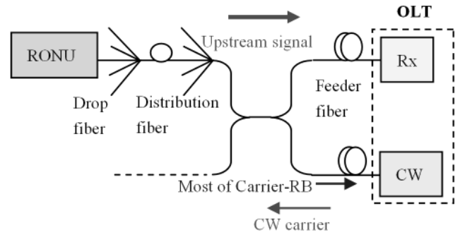
Fig. 4. Schematic of a carrier distributed PON using dual-feeder fiber architecture.
