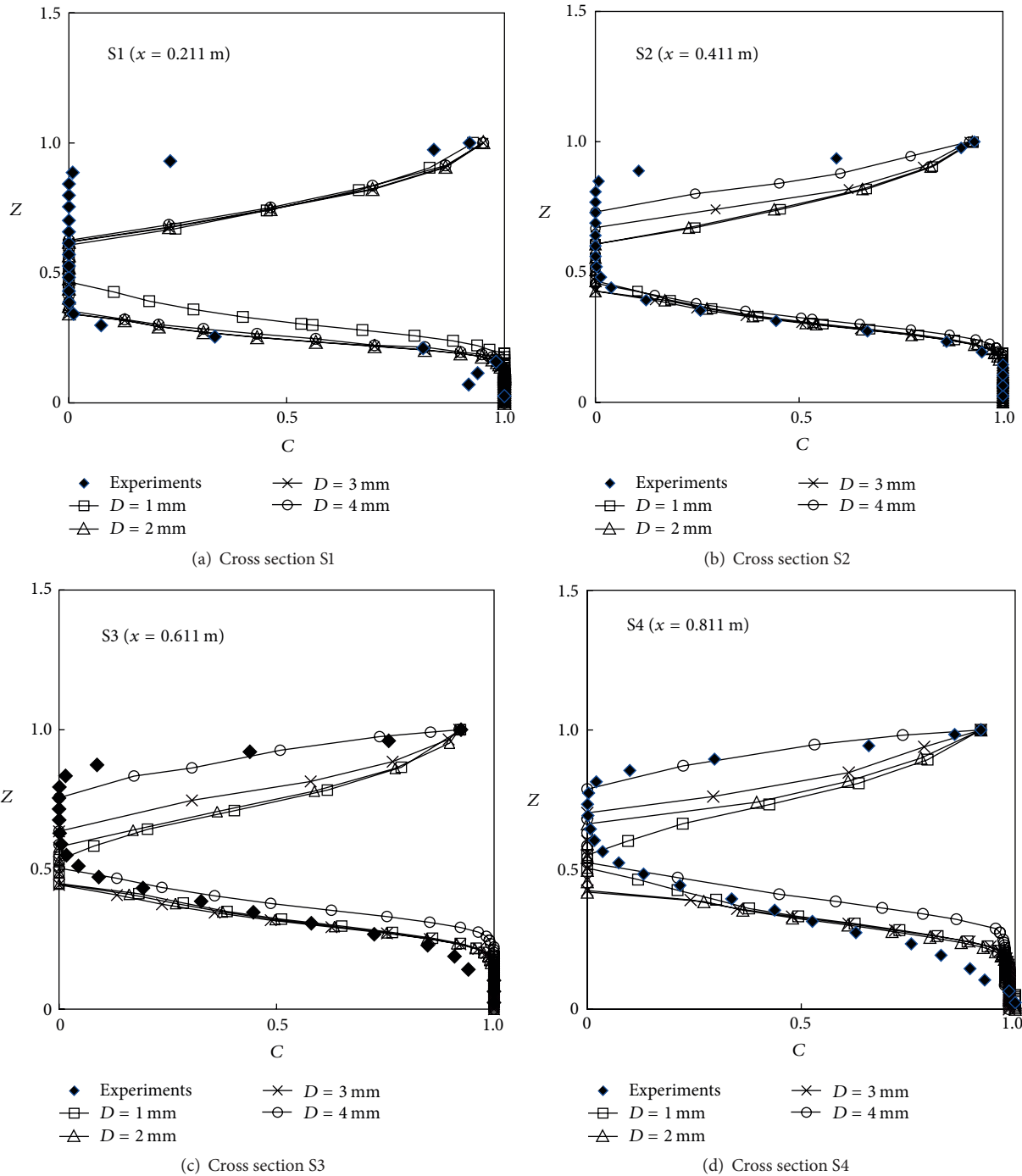
FIGURE 6: C distributions.
