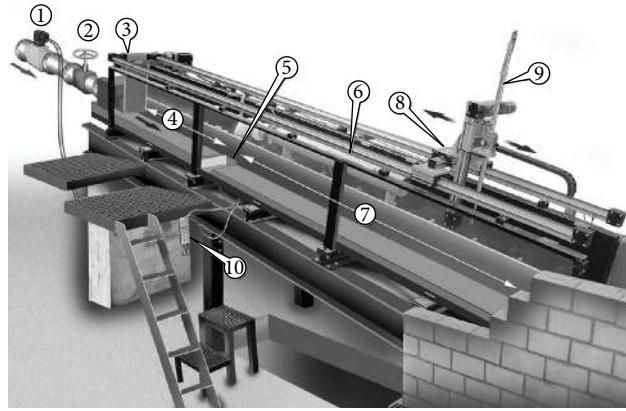
FIGURE 1: Chute model configuration [7] (with permission from ASCE). (1) flow meter, (2) slide valve, (3) jet-box, (4) approach flow zone, (5) aerator, (6) air duct, (7) measurement range, (8) automatic position system, (9) fiber-optical probe, and (10) cavity piezometer.
