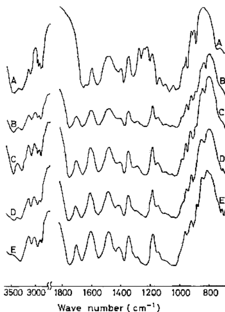
Figure 1. Infrared absorption spectra of chitin and acetylchitins: A, chitin; B, 1.1 acetylchitin; C, 1.4 acetylchitin; D, 1.7 acetylchitin; E, diacetylchitin.
