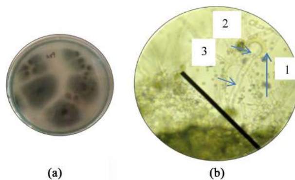
Figure 2. (a) Macroscopic and microscopic Aspergillus sp. , green color of colony, (b) Morphology of Aspergillus with magnification 40× (1) conidiospore, (2) vesicle, (3) conidiophore.
