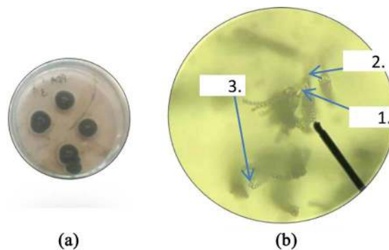
Figure 3. (a) Macroscopic and microscopic Penicillium sp. , old green colour of colony, (b) Morphology of Penicillium sp. with magnification 40× (1) Phialide, (2) conidiophore, (3) conidium.
