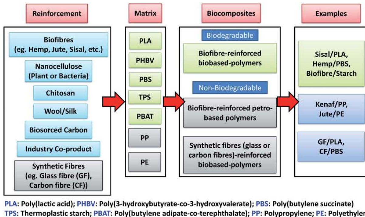
Fig. 1 Types of biocomposites and examples.
