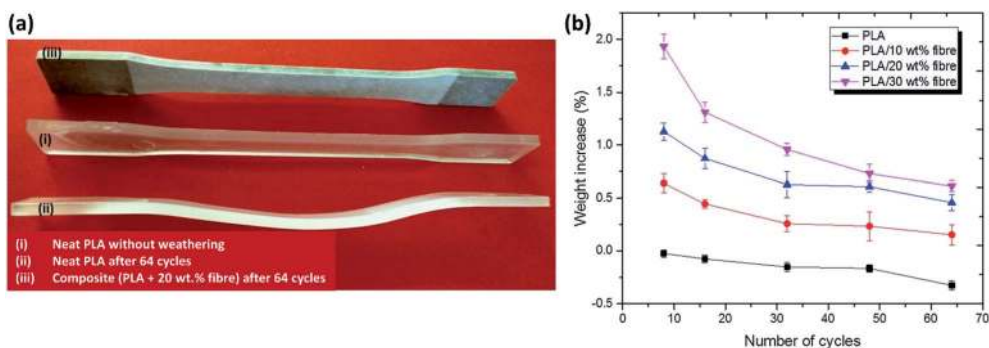
Fig. 14 Effect of accelerated weathering aging cycles (UV light, water spray and condensation according to ASTM G154) on PLA and its biocomposites on (a) dimension changes and (b) weight changes. This figure has been reproduced with permission from ref. 85, SpringerLink, Copyright 2019 (License Number: 4710330395191).
