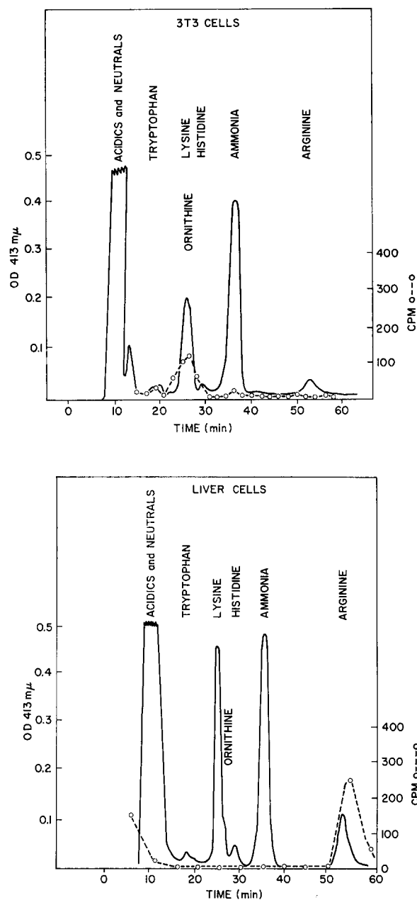
FIGURE 3 Assay for the transformation of ornithine- 3 H into arginine- 3 H. Cells to be tested were incubated in the presence of ornithine- 3 H in arginine-deficient medium for 24 hr. The cells were washed, dissolved in 6 N HCl, and hydrolyzed. The dried sample was dissolved in the appropriate buffer, and amino acid analysis was performed as described in Materials and Methods. The elution volume was collected in 2 ml fractions, and the radioactivity was determined in a liquid scintillation counter. (a) 3T3 cells; (b) fetal rat liver cells. Abscissa: time after starting the fractionation, in minutes (fraction number [elution volume]). Ordinates: (left) OD413 mμ; (right) counts per minute.
