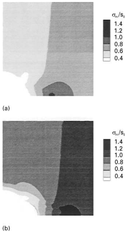
Figure 14 Distribution of the hydrostatic mean stress, \sigma_m , for the same material as in Fig. 13 but for high triaxiality loading, \Sigma_1/\Sigma_2 = 0.73 , under (a) plane strain, E_c = 0.043 , and (b) axisymmetric conditions, E_c = 0.040 .
