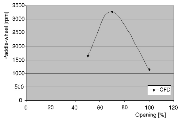
Variation of paddle-wheel rpm with port opening for ALE2 engine – CFD results (5.74 mm valve lift)
