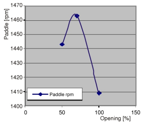
Variation of paddle-wheel rpm with port opening for W06DTIE2 engine – Experimental results
