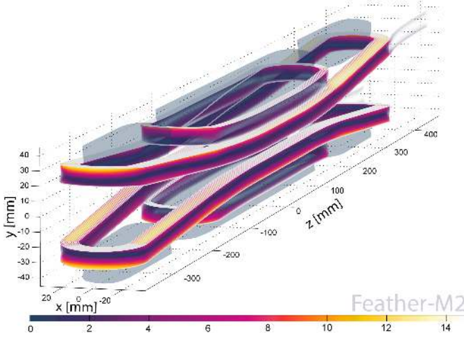
Fig. 7. Three dimensional coil layout and incident angle of the magnetic field plotted on the conductor for the Feather-M2 when operated in a background field of 13 T.
