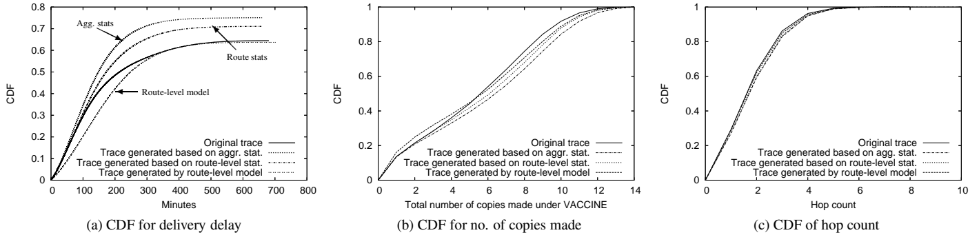
Figure 11: Comparison of epidemic routing performance under original trace and synthetic traces generated by three different models
