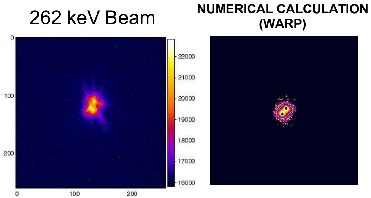
Figure 15: Analog (pinhole) simulation and WARP3D calculation of fully neutralized beam focused to a small spot. Image box size is 4cm \times 4 cm squares.
