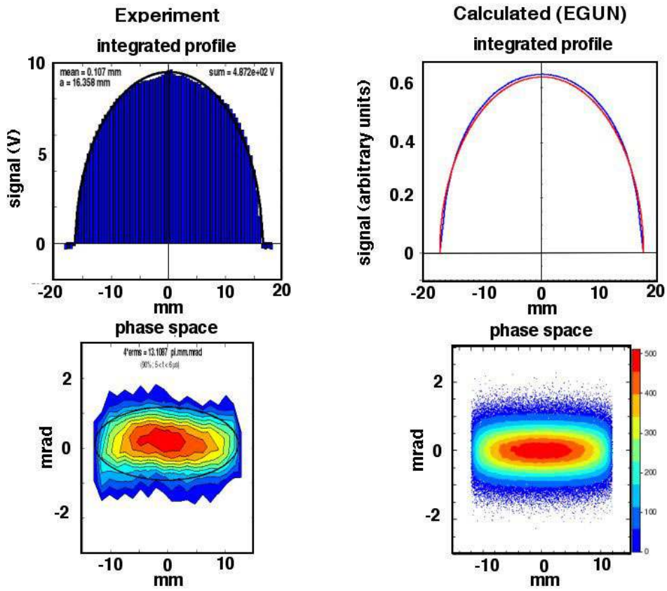
Figure 7: Slit-integrated density profile and (x, x') phase space of a high-brightness apertured beam (300kV, 25 mA, 2-cm aperture diameter). The corresponding EGUN calculations are shown to the right.
