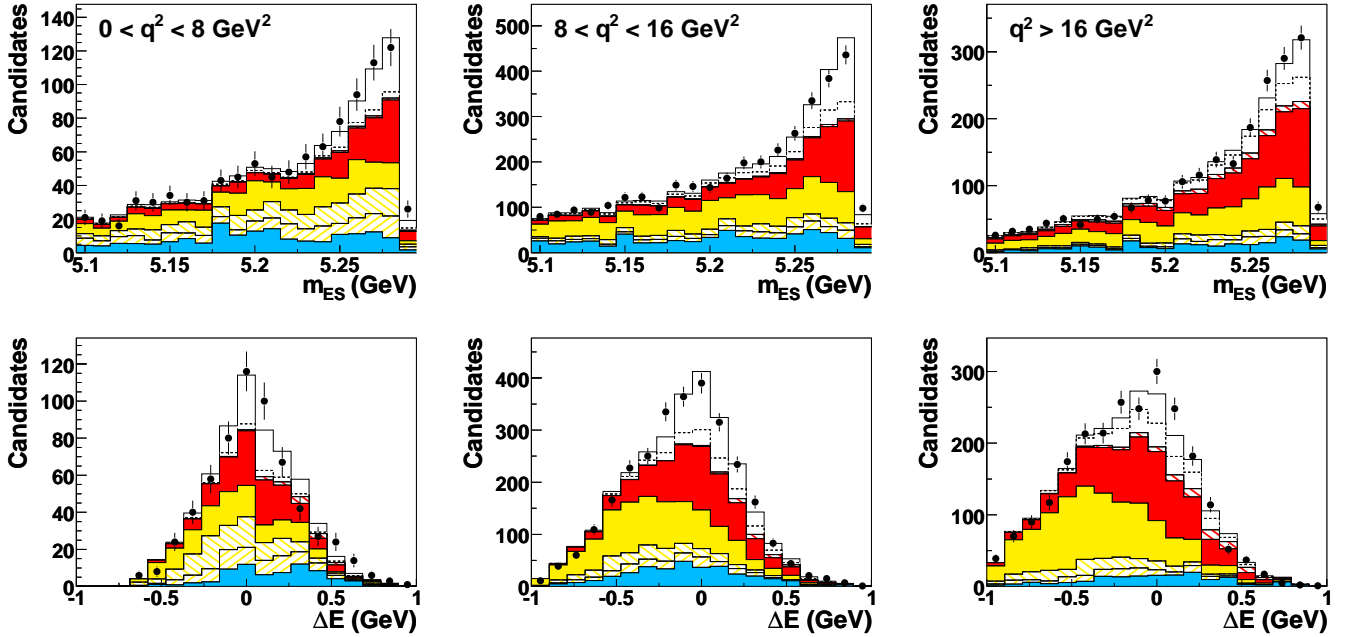
FIG. 23: (color online) m_{\text{ES}} and \Delta E distributions in each q^2 bin for B^+ \rightarrow \rho^0 \ell^+ \nu after the fit. The distributions are shown in the \Delta E and m_{\text{ES}} signal bands, respectively. Legend: see Figure 5.
