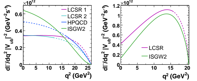
FIG. 2: q^2 distributions for B \rightarrow \pi \ell \nu (left) and B \rightarrow \rho \ell \nu (right) decays, based on form-factor predictions from the ISGW2 model [14], LCSR calculations (LCSR 1 [15] and LCSR 2 [19] for B \rightarrow \pi \ell \nu and LCSR [17] for B \rightarrow \rho \ell \nu ) and the HPQCD [23] lattice calculation. The extrapolations of the QCD predictions to the full q^2 range are marked as dashed lines.
