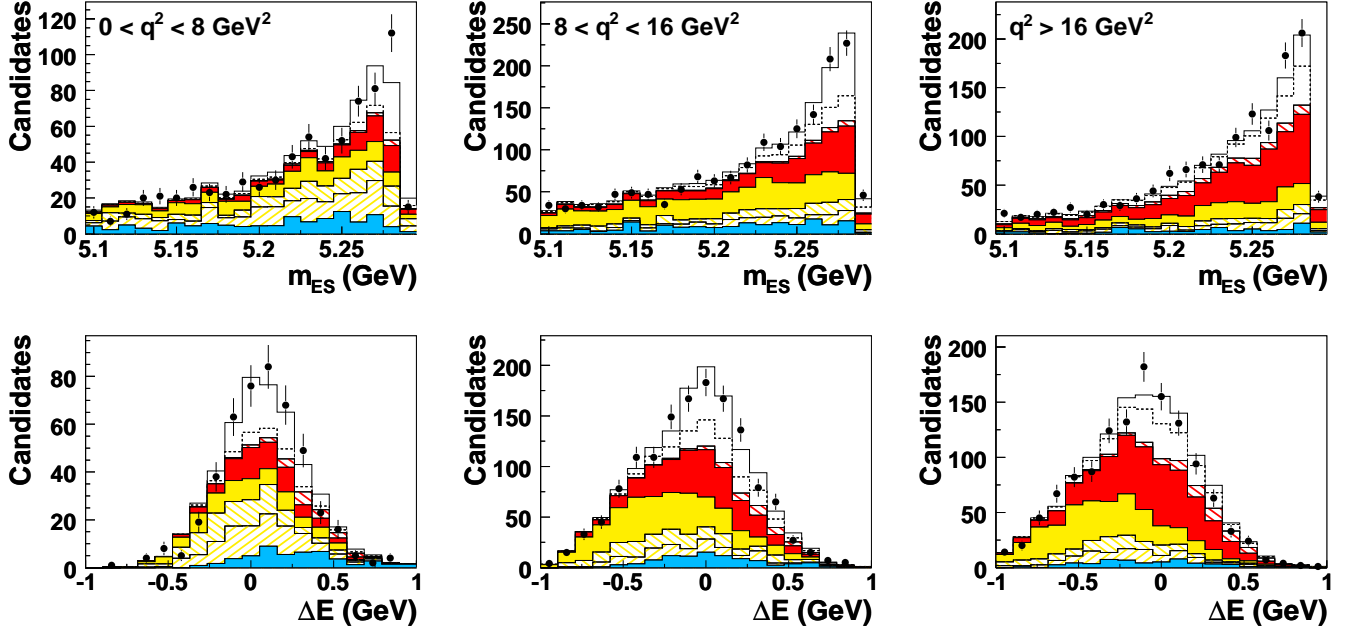
FIG. 22: (color online) m_{\text{ES}} and \Delta E distributions in each q^2 bin for B^0 \rightarrow \rho^- \ell^+ \nu after the fit. The distributions are shown in the \Delta E and m_{\text{ES}} signal bands, respectively. Legend: see Figure 5.
