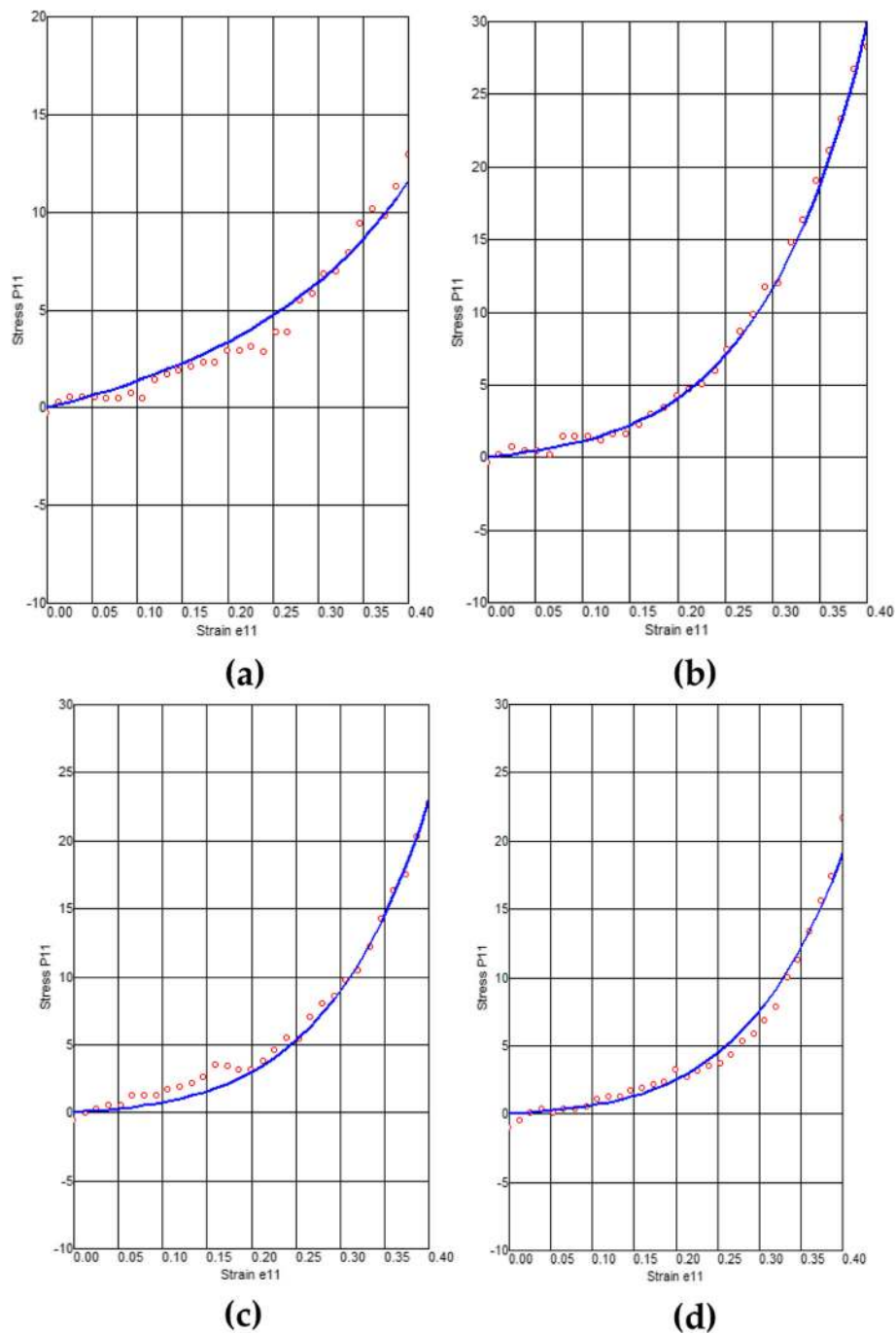
Fig. 4 Curve fitting of experimental data versus the Fung model on the RV sample cut for biaxial testing. a RV sample 1, b RV sample 2, c RV sample 3 and d RV sample 4. Unit for Stress P11 is kPa and Strain E11 is mm/mm
