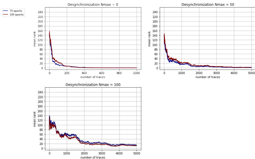
Figure 34: Mean ranks of CNN_{best} for a desynchronization amount in \{0, 50, 100\} .
