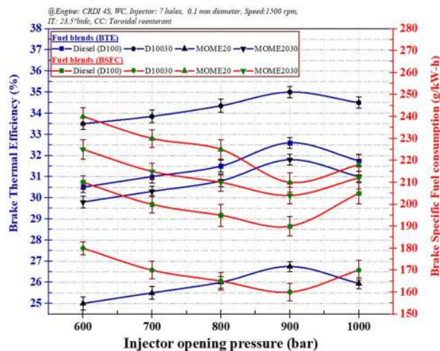
Figure 4. The variation of injection opening pressure: (a) brake specific fuel consumption, and (b) brake thermal efficiency.
