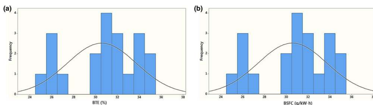
Figure 6. Variation of frequency with: (a) brake thermal efficiency and (b) brake specific fuel consumption.
