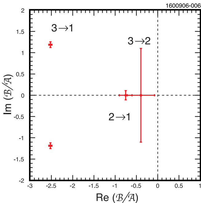
FIG. 12 (color online). Complex values of matrix element ratio B/\mathcal{A} from combined fits for the three transitions under the assumption that C=0 . Note the twofold ambiguity in the imaginary part.
