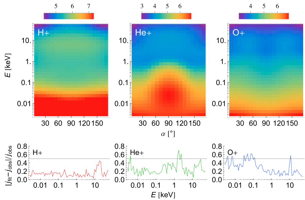
Figure 4. (top) Fitted ion distributions using multiples of equation (1), and (bottom) median values of relative errors of the fitting in each energy channel. Left, middle, and right columns correspond to H+, He+, and O+ ions, respectively.
