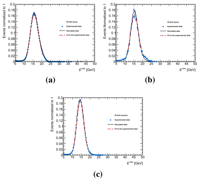
Fig. 18 Distributions of the reconstructed energy E^{\text{raw}} obtained analyzing pion (a), kaon (b) and proton (c) data with E_{\text{beam}} = 20 GeV. The blue dotted histograms represent the experimental data. Only statistical uncertainties are shown. The dashed curves in red correspond to the fit of a Gaussian function to the experimental data in a region \pm 2\sigma around the peak value. The black histograms correspond to the predictions of the MC simulation
