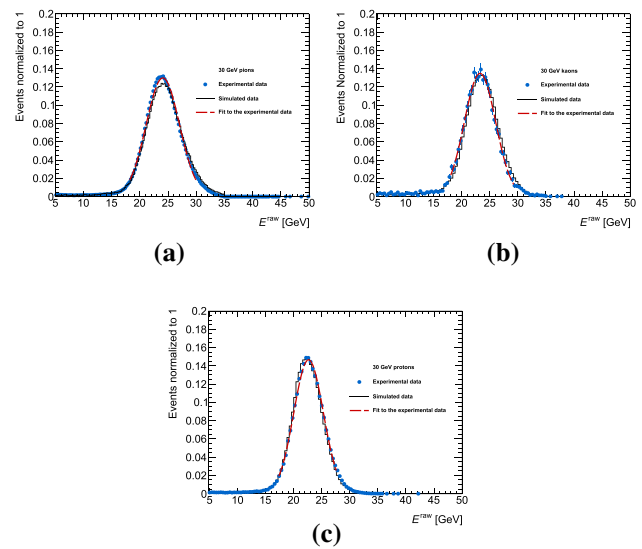
Fig. 19 Distributions of the reconstructed energy E^{\text{raw}} obtained analyzing pion (a), kaon (b) and proton (c) data with E_{\text{beam}} = 30 GeV. The blue dotted histograms represent the experimental data. Only statistical uncertainties are shown. The dashed curves in red correspond to the fit of a Gaussian function to the experimental data in a region \pm 2\sigma around the peak value. The black histograms correspond to the predictions of the MC simulation
