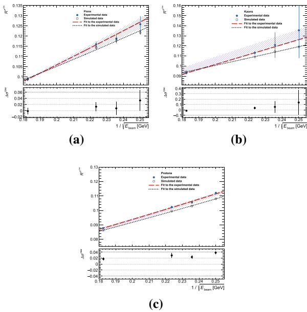
Fig. 21 Energy resolution normalized to incident beam energy, R^{\sigma^{\text{raw}}} , measured (blue circles) and predicted by MC simulation (black circles) as a function of 1/\sqrt{E_{\text{beam}}} obtained in the case of pion (a), kaon (b) and proton (c) beams. The experimental uncertainties include statistical and systematic effects combined in quadrature. Only statistical uncertainties affect simulated results. The red dashed (black dotted) curves are fits to the experimental (simulated) data points. In case of experimental determinations the dashed blue hashed bands were obtained by using the correlated systematic uncertainties. In the bottom of the histograms are shown the fractional differences \Delta\sigma^{\text{raw}} defined in Eq. (13). The uncertainty includes statistical and systematic effects combined in quadrature
