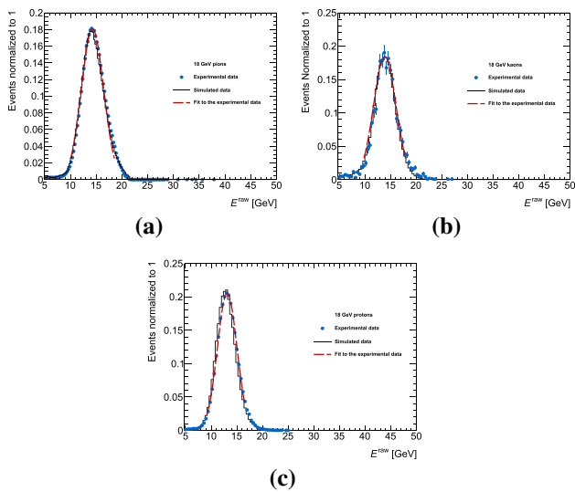
Fig. 17 Distributions of the reconstructed energy E^{\text{raw}} obtained analyzing pion (a), kaon (b) and proton (c) data with E_{\text{beam}} = 18 GeV. The blue dotted histograms represent the experimental data. Only statistical uncertainties are shown. The dashed curves in red correspond to the fit of a Gaussian function to the experimental data in a region \pm 2\sigma around the peak value. The black histograms correspond to the predictions of the MC simulation
