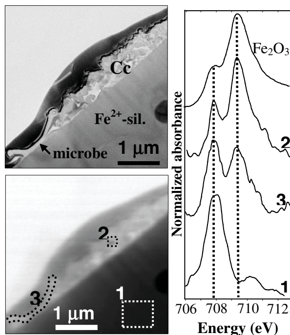
FIGURE 4. (Upper left) TEM image of a cross-section showing a microorganism (arrow), a calcite crystal cluster (Cc), and a \text{Fe}^{2+} -silicate. (Bottom left) Equivalent STXM image at 707.8 eV. (Right) Iron L_3 -edge NEXAFS spectra from the silicate (area 1), the calcite cluster (area 2), the microorganism (area 3), and reference hematite, representing the \text{Fe}^{3+} endmember. Dashed lines represent the positions of \text{Fe } L_3 maxima for \text{Fe}^{2+} and \text{Fe}^{3+} at 707.8 and 709.5 eV, respectively. (from [16])
