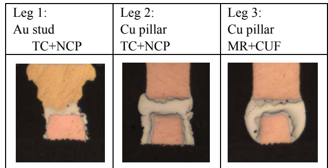
Figure 9 : X-section view of bumps
