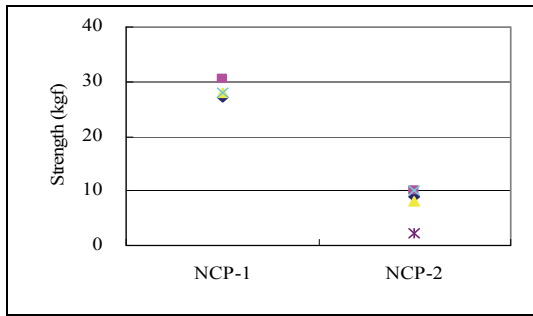
Figure 7 : Adhesion strength of NCP on die
