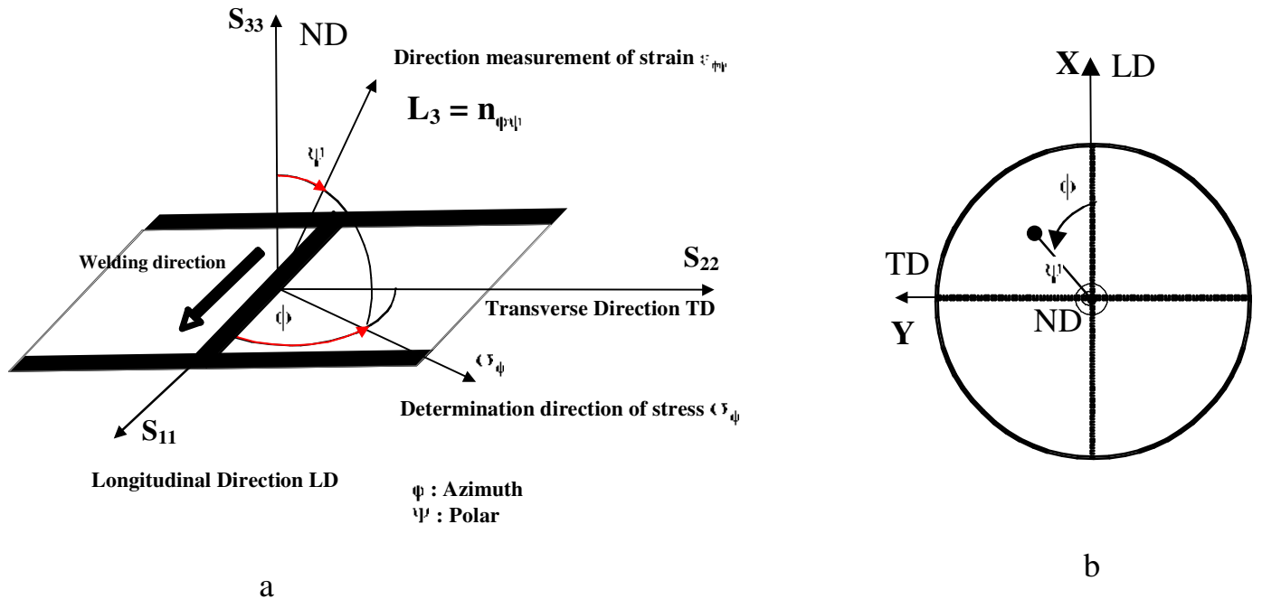
Figure 1: (a) Orientation of strain components \varepsilon_{\phi\psi} and of the stress components \sigma_{\phi} with respect to the coordinate system S_{11} , S_{22} , S_{33} of the sample and (b) those of the sample for the areas measured.
