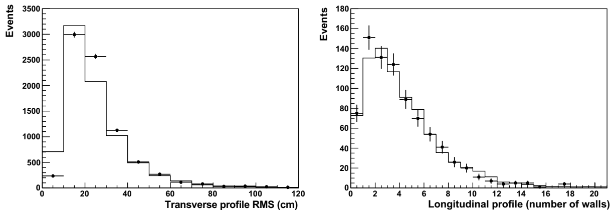
Figure 12. Transverse hadronic shower profile (left), in the X and Y projections, and longitudinal profile (right), in the number of TT walls. Data are shown by dots with error bars and MC by the solid line. MC distributions are normalized to data.
