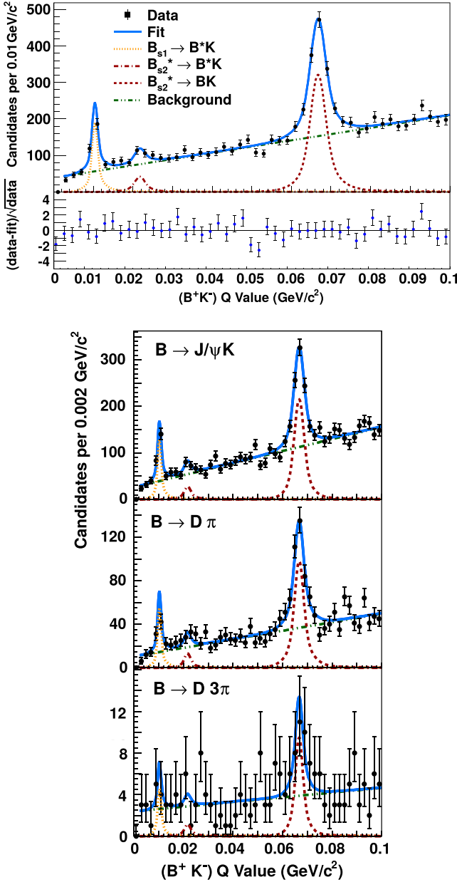
FIG. 5 (color online). Distribution of the Q value of B_s^{*0} candidates with fit results overlaid. The upper panel shows the data summed over decay channels and the deviations of these from the fit function, normalized to the Poisson uncertainty of the data. The lower panels show data and fits for each decay channel individually.
