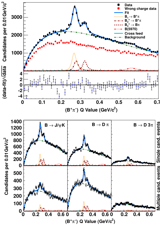
FIG. 3 (color online). Distribution of the Q value of B^{*0} candidates (and B^+\pi^+ combinations in the upper plot) with fit results overlaid. The upper panel shows the data summed over decay channels and the deviations of these from the fit function, normalized to the Poisson uncertainty of the data. The lower panels show data and fits for each decay channel individually, separated into events with one candidate (upper row) and with multiple candidates (lower row).
