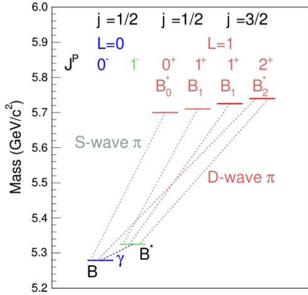
FIG. 1 (color online). Spectrum and allowed decays for the lowest orbitally excited states B^{**0,+} . For B_s^{**0} mesons the pion is replaced by a kaon and the states have higher masses.
