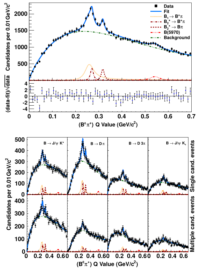
FIG. 4 (color online). Distribution of the Q value of B^{*+} candidates with fit results overlaid. The upper panel shows the data summed over decay channels and the deviations of these from the fit function, normalized to the Poisson uncertainty of the data. The lower panels show data and fits for each decay channel individually, separated into events with one candidate (upper row) and with multiple candidates (lower row).
