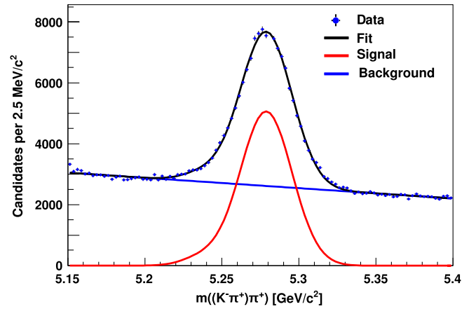
FIG. 2 (color online). Invariant K\pi\pi -mass distribution of B^+ \rightarrow \bar{D}^0 (\rightarrow K^- \pi^+) \pi^+ candidates after the application of loose requirements, before neural network selection, with fit result overlaid.
