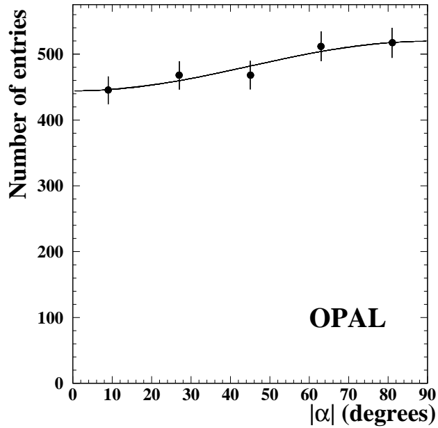
Figure 5: The |\alpha| distribution of background subtracted D^* candidates for x_E > 0.5 , fitted to N(1 + 2\text{Re} \rho_{1-1} \cos 2|\alpha|) , where the overall normalisation factor N and the matrix element \text{Re} \rho_{1-1} are free parameters.
