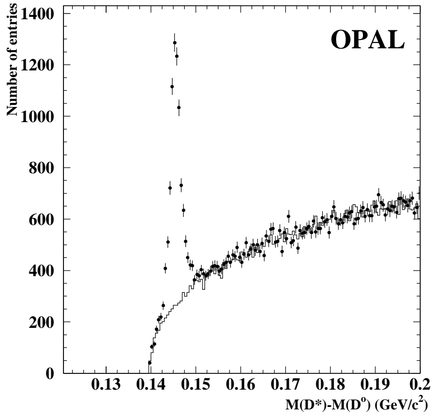
Figure 3: Mass difference distribution for the D^* candidates with x_E > 0.2 , before applying the \Delta M cut. The points show the signal sample and the line histogram the distribution of the background obtained from wrong-charge, reflected pion and reflected pion wrong-charge combinations. The errors on the data points are statistical only.
