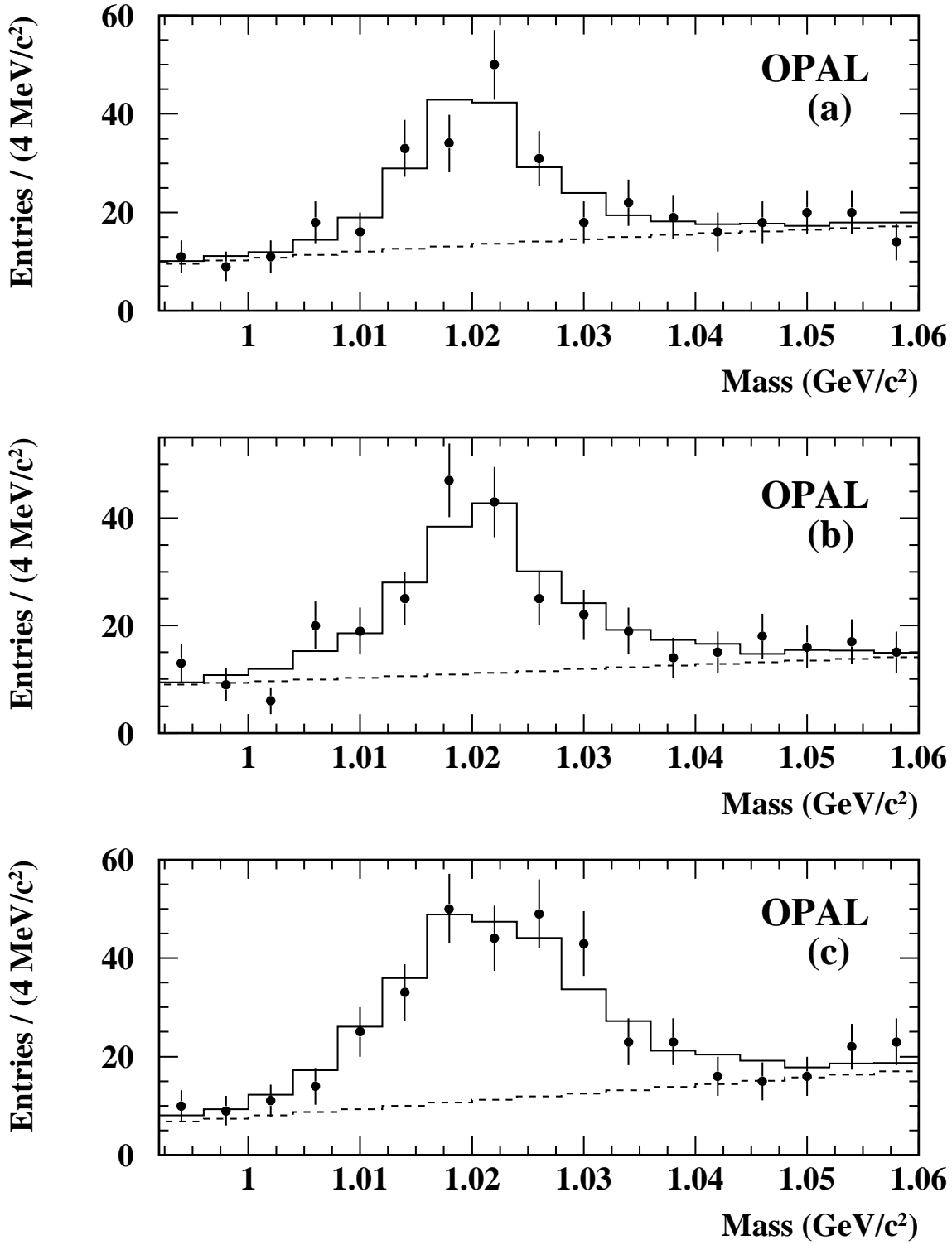
Figure 1: Two-particle invariant mass distribution of K^+K^- pairs with x_E > 0.7 in the ranges of decay angle (a) 0 \leq |\cos \theta_H| < 1/3 , (b) 1/3 \leq |\cos \theta_H| < 2/3 and (c) 2/3 \leq |\cos \theta_H| \leq 1 . The points with error bars are the data. The solid histograms show the fits, with the background components shown separately as dashed histograms.
