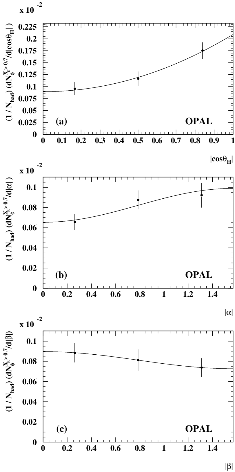
Figure 2: Corrected differential rates for \phi mesons fitted to (a) N(1 - \rho_{00} + (3\rho_{00} - 1) \cos^2 \theta_{\text{H}}) , (b) N(1 + 2 \operatorname{Re} \rho_{1-1} \cos 2|\alpha|) , (c) N(1 + 2 \operatorname{Im} \rho_{1-1} \cos 2|\beta|) , where the overall normalisation factors N and the spin density matrix elements are free parameters in the fits.
