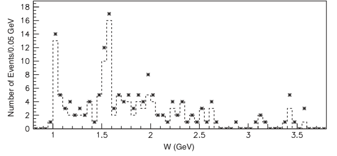
FIG. 3. The experimental W distributions of the signal candidates at 2 \text{ GeV}^2 < Q^2 < 30 \text{ GeV}^2 ( 3 \text{ GeV}^2 < Q^2 < 30 \text{ GeV}^2 ) as indicated by the asterisks (dashed histogram). Backgrounds have not been subtracted.
