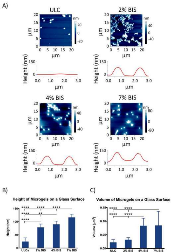
Figure 4. (a) AFM scans and corresponding representative height traces for each microgel type after deposition on a glass coverslip. (b) Average height of each microgel type after deposition on a glass surface. (c) Average volume of each microgel type, obtained from height and spread areas of each microgel type after deposition on a glass surface. A minimum of 30 particles were analyzed per microgel type. Error bars represent standard deviations from the mean. **: p < 0.01 ; ****: p < 0.0001 .
