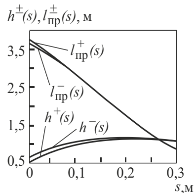
Figure 7. Graphs h^\pm, l_{пп}^\pm \sim s for s = 0,01 \text{ m} and nstep = 30 .
