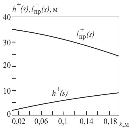
Figure 15. Graphs h^{\pm}, l_{np}^{\pm} \sim s .
