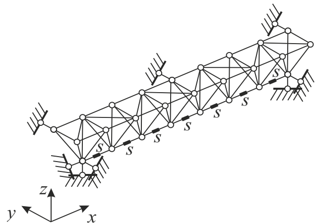
Figure 1. Initial state of the truss.
