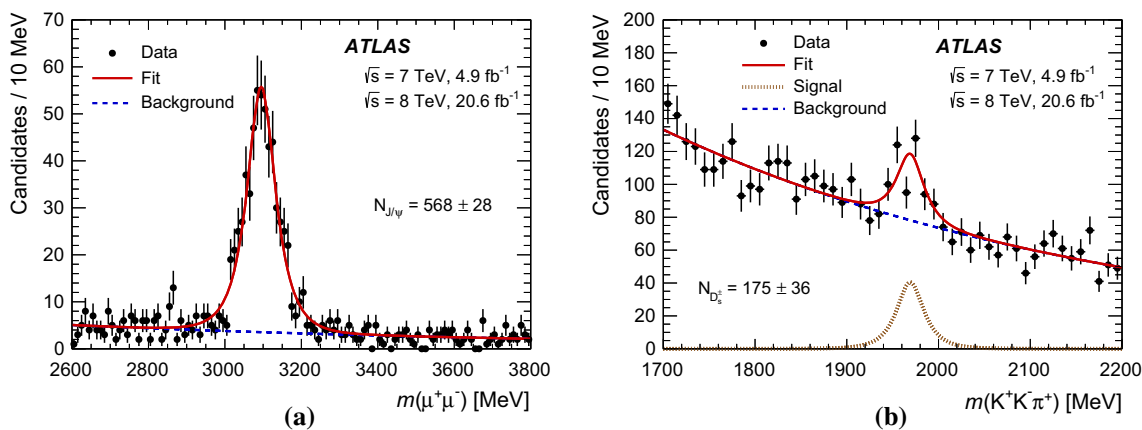
Fig. 4 Mass distribution of the a J/\psi and b D_s^+ candidates after the full B_c^+ \rightarrow J/\psi D_s^{*+} selection (without mass constraints in the cascade fit) in the mass window of the B_c^+ candidate 5900 \text{ MeV} <
