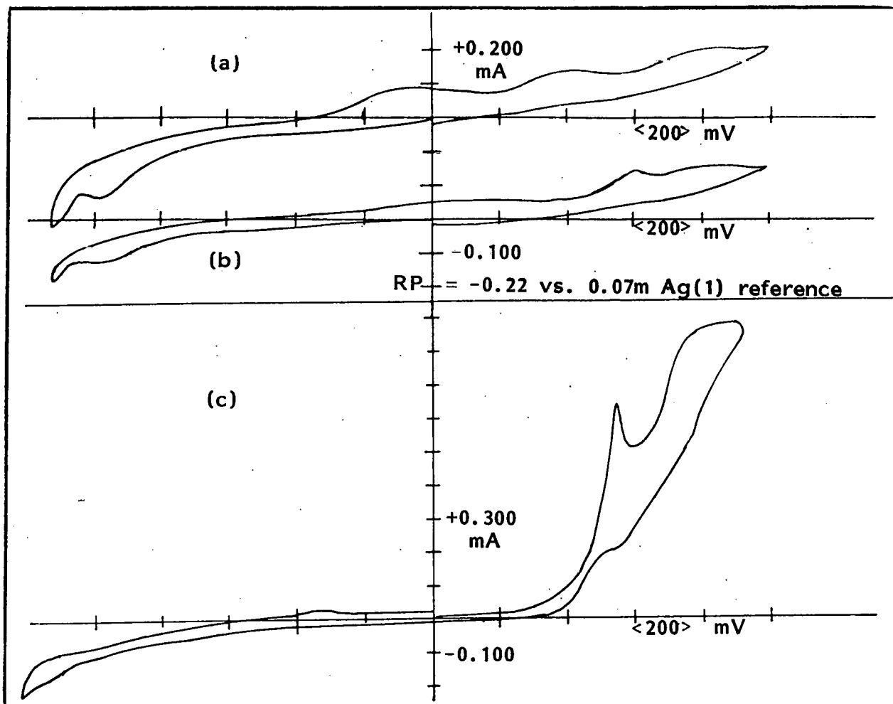
Fig. 48a. Cyclic voltammogram showing background during removal of \text{CO}_2/\text{water} : v = 0.100 \text{ V-sec}^{-1} , T = 300^\circ\text{C} (20 min after dry argon introduced). 48b. Cyclic voltammogram showing background 15 hours after dry argon: v = 0.100 \text{ V-sec}^{-1} , T = 300^\circ\text{C} . 48c. Cyclic voltammogram after addition of 30.8 \times 10^{-3} molal \text{NaNO}_2 and 12.5 \times 10^{-3} molal \text{K}_2\text{CO}_3 : v = 0.100 \text{ V-sec}^{-1} , T = 300^\circ\text{C} .
