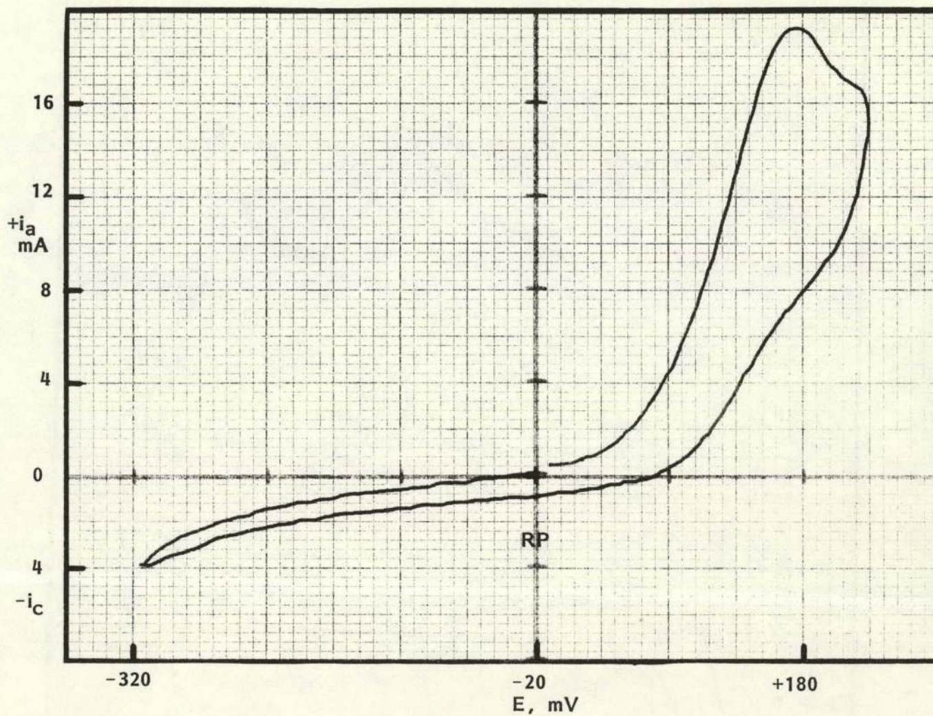
Fig. 46. Anodic peak observed after \text{CO}_2 in contact with nitrate melt after 3 days. E vs. \text{Ag}/\text{Ag}(1) 0.07m reference. Scan rate = 1.0 \text{ V}\cdot\text{sec}^{-1} .
