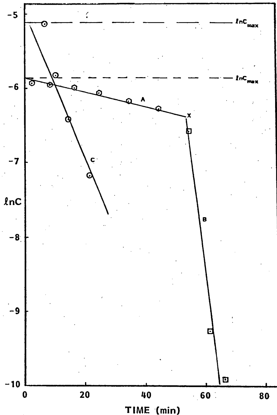
Fig. 36. Plot of log water concentration (mol·kg -1 ) versus time in min.
