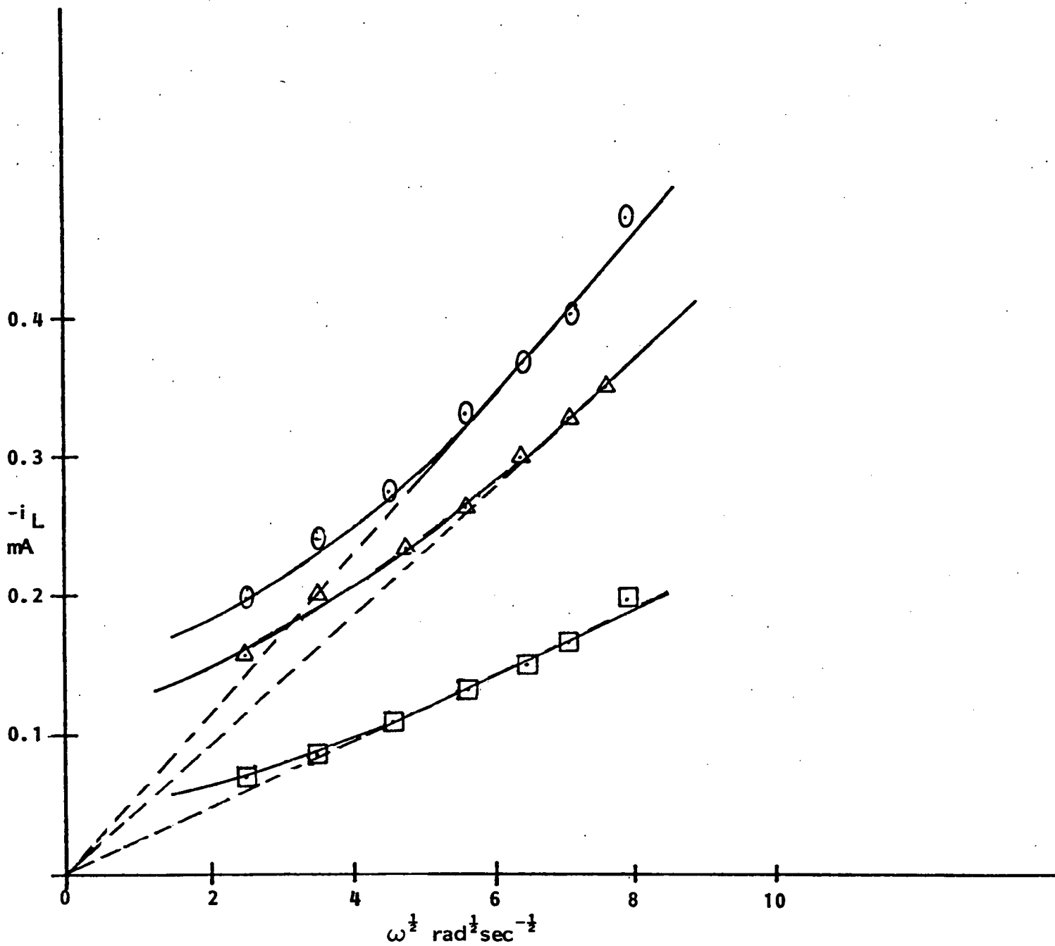
Fig. 29. Plot of -i_L /mA versus the square root of the rotation rate at 295°C and three water partial pressures: ○, 18.20 mm; △, 12.38 mm; and □, 7.51 mm. Au disc = 0.021 cm 2 .
