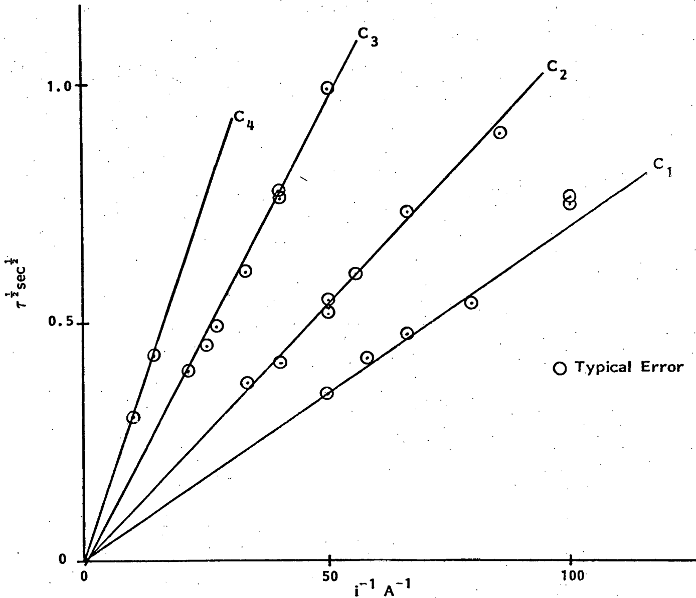
Fig. 40. Sand's plot for carbonate ion oxidation at 505^\circ\text{C} . Gold electrode, 0.21 \text{ cm}^2 .
