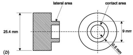
Fig. 3 Drawing of the cup-shaped 1018 steel piece for (a) the case of large contact area and (b) the case of small contact area
