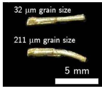
Fig. 1 Samples of pins extruded using the 0.76:0.57 mm die and work pieces having a grain size of 32 \mu\text{m} and 211 \mu\text{m} (modified from [2])
