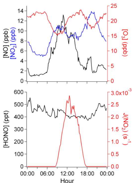
Fig. 4. Average diurnal 10 min profiles for O_3 , NO_x , HONO, and J(NO_2) during the MEGAPOLI winter campaign (local time).
