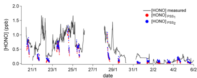
Fig. 7. Observed HONO mixing ratios (black lines) compared with PSS calculations (red circles for Eq. 1 and blue circles for Eq. 2) for the MEGAPOLI winter campaign. The calculations with the PSS approach are carried out only when all the parameters used in it are available.
