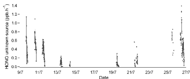
Fig. 9. Evolution of the calculated unknown HONO source in \text{ppb h}^{-1} (Eq. 4) during the MEGAPOLI summer campaign.
