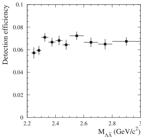
FIG. 10. The \Lambda\bar{\Lambda} mass dependence of detection efficiency obtained from MC simulation.
