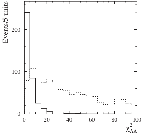
FIG. 26. The \chi_{\Lambda\Lambda}^2 distributions for simulated e^+e^- \rightarrow \Lambda\bar{\Lambda}\gamma events (solid histogram) and e^+e^- \rightarrow \Lambda\bar{\Sigma}^0\gamma events (dashed histogram).
