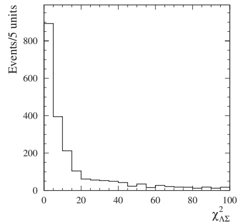
FIG. 25. The \chi^2_{\Lambda\Sigma} distributions for simulated e^+e^- \rightarrow \Lambda\bar{\Sigma}^0\gamma events.
