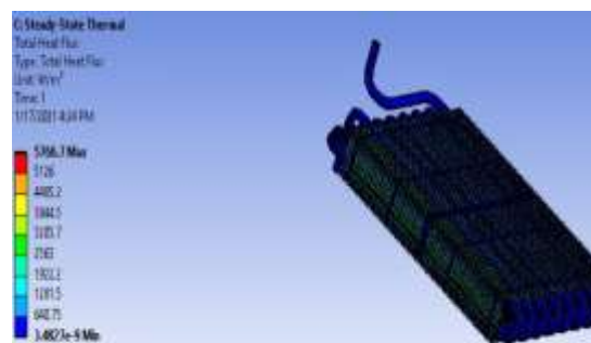
Figure-4(k): Total heat flux variation for tube copper, fins Al alloy 7050 and R32
