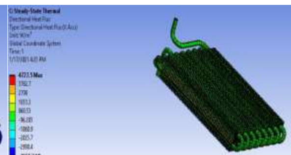
Figure-4(l): Directional heat flux variation for tube copper, fins Al alloy 7050 and R32
