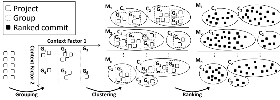
Fig. 8 Steps to train a universal defect prediction model.
