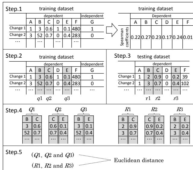
Fig. 3 The five steps in the technique for calculating the domain-agnostic similarity between two projects.
