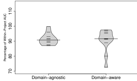
Fig. 5 The impact of metrics for calculating domain-aware similarity.
