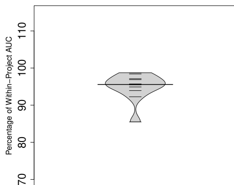
Fig. 10 [RQ3-1] The results of our simple voting approach.
