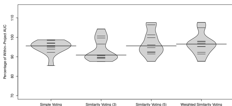
(b) Domain-aware
