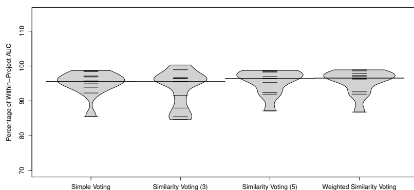
(a) Domain-agnostic
