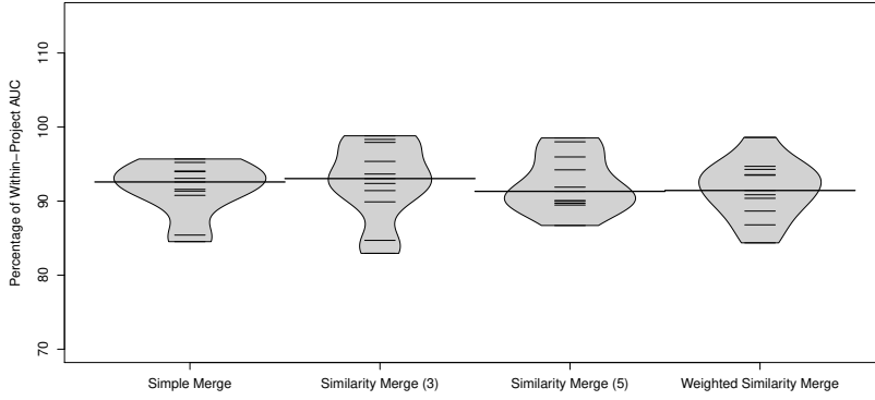
(a) Domain-agnostic
