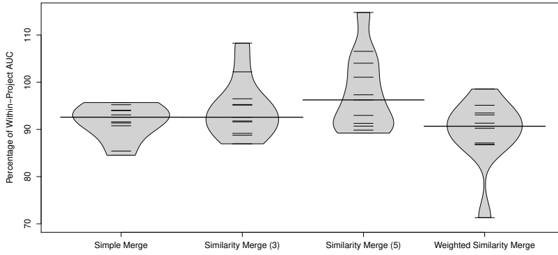
(b) Domain-aware
