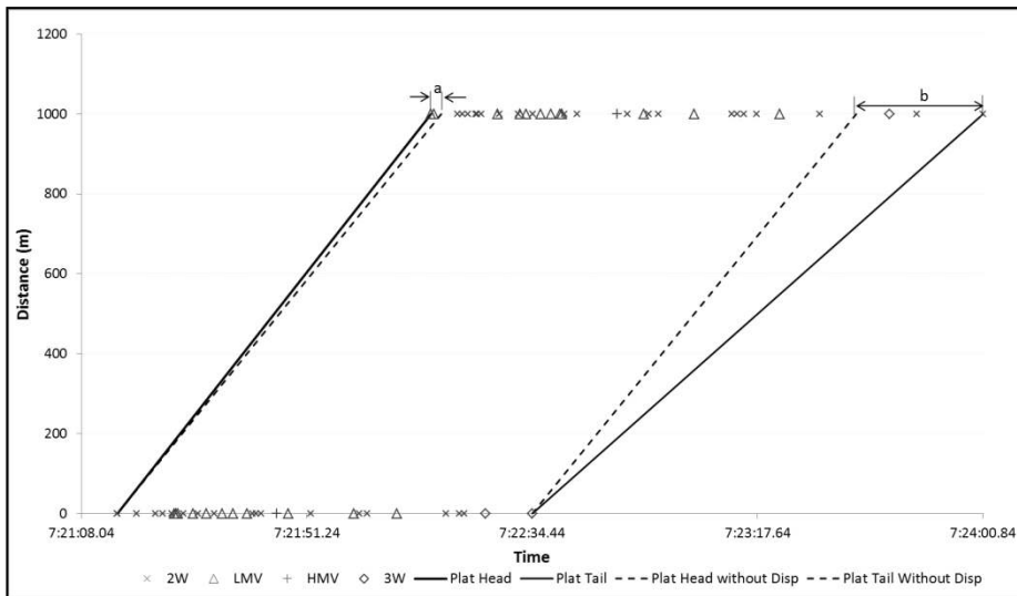
Fig. 3. Dispersion of platoon from upstream to downstream
