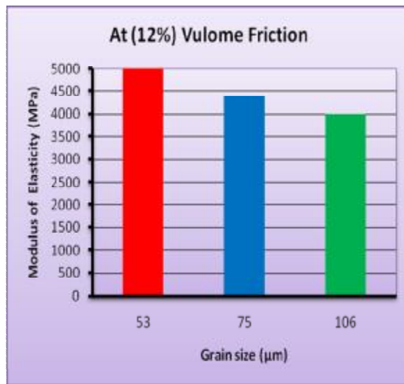
Figure (5): shown the effect of particle size on young's modulus at volume fraction of (12%).
