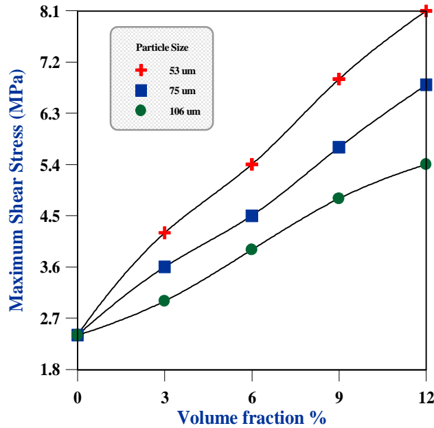
Figure (8): shown the effect of volume fraction on maximum shear stress
