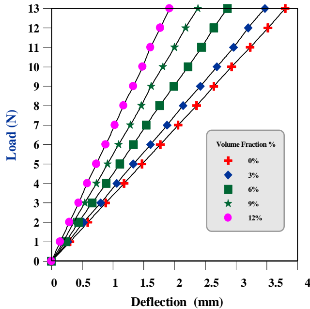
Figure (3): shown the effect of load on deflection for varying volume fraction with a particle size of (106 μm).
