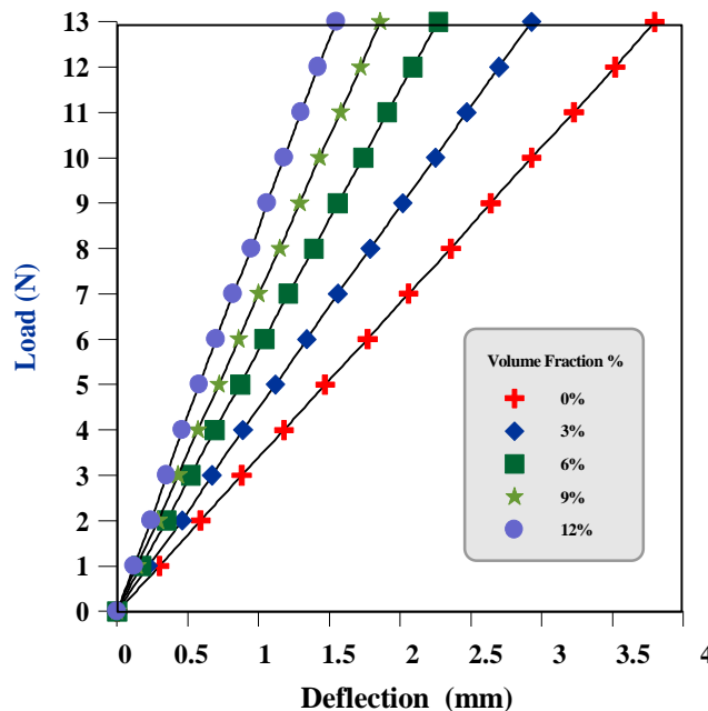
Figure(1): shown the effect of load on deflection for varying volume fraction with a particle size of (53 μm).
