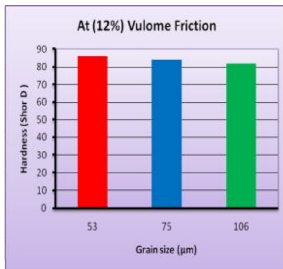
Figure (11): shown the effect of particle size on the hardness at volume fraction of (12%).
