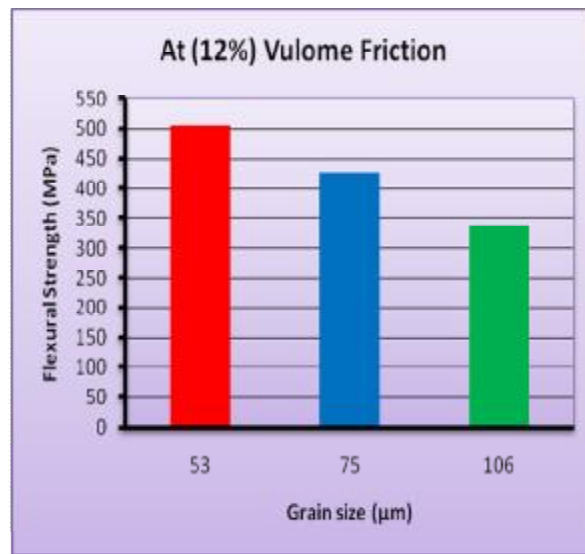
Figure (7): shown the effect of particle size on Flexural strength at volume fraction of (12%).
