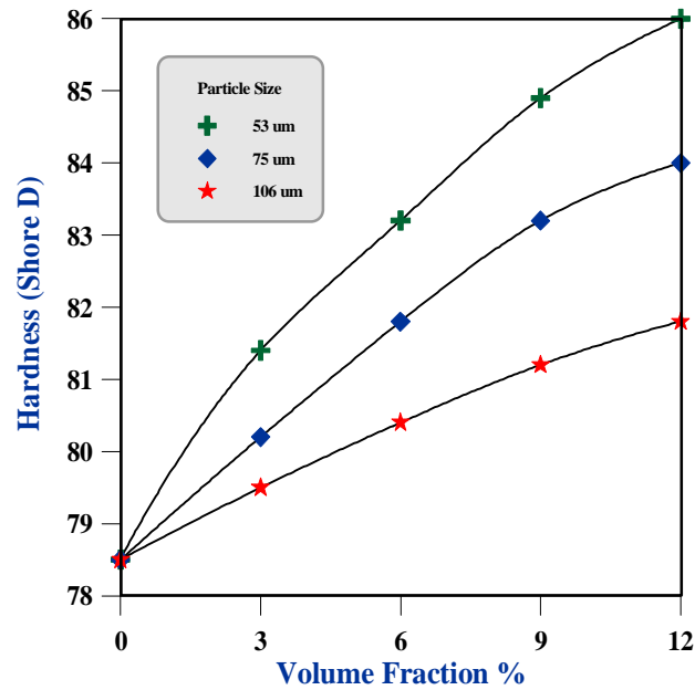
Figure (10): shown the effect of volume fraction on hardness
