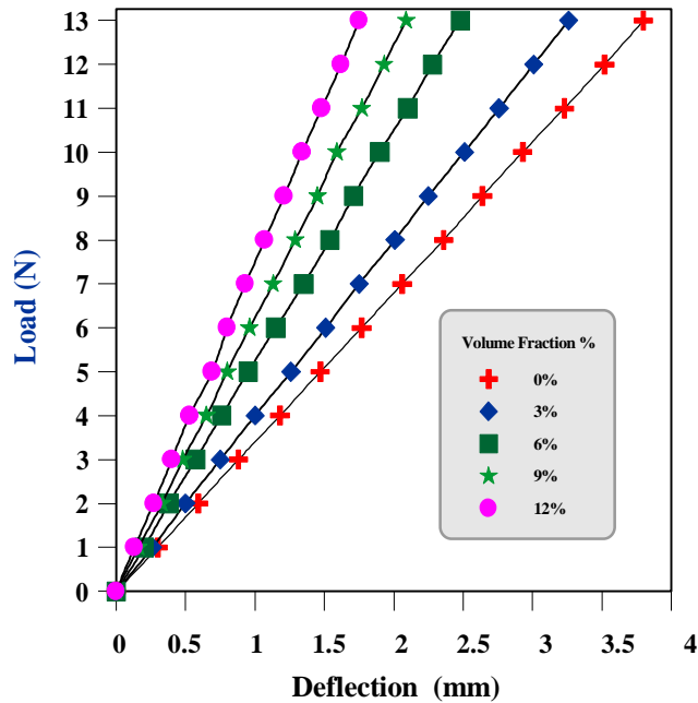
Figure (2): shown the effect of load on deflection for varying volume fraction with a particle size of (75 μm).
