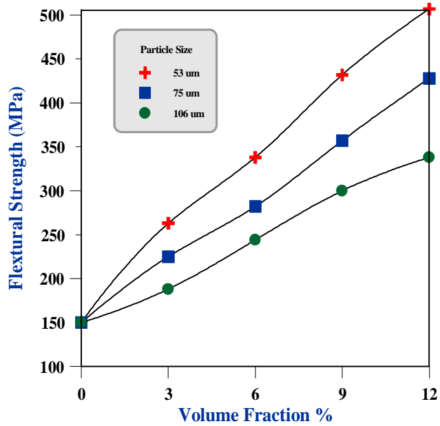
Figure (6): shown the effect of volume fraction on flexural strength.
