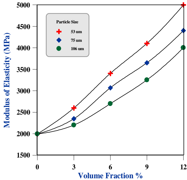
Figure(4): shown the effect of volume fraction on young's modulus.
