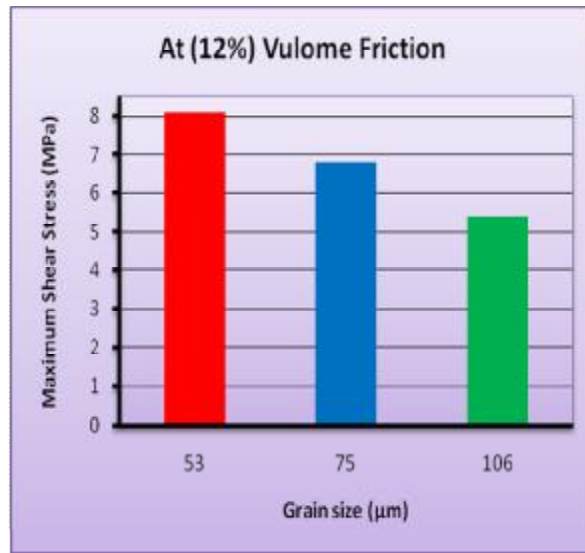
Figure (9): shown the effect of particle size on maximum shear stress at volume fraction of (12%).
