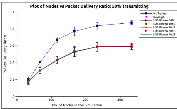
Fig. 7. Impact of the Rician K -Factor on PDR
