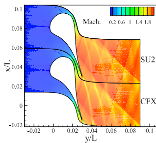
Figure 7: Mach contour.
