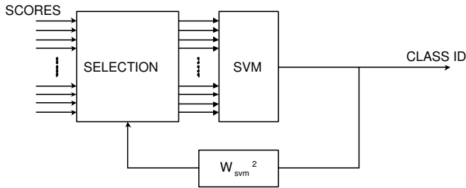
Fig. 2. Diagram of a Recursive Band Elimination Method
