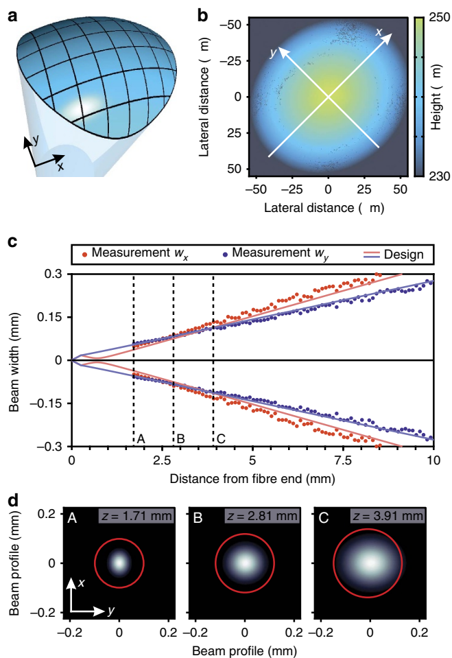
Figure 3 | Toric lens for the generation or the correction of astigmatism.
