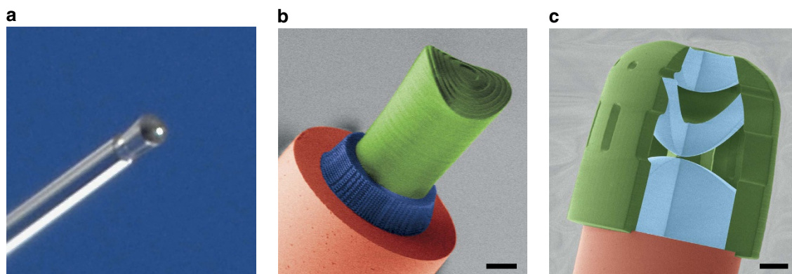
Figure 1 | Polarization controlling, diffractive, refractive and imaging optical elements directly attached to the end facet of an optical fibre. (a) Macro photograph of a lens that collimates a Gaussian beam emerging from a single-mode fibre. (b) Coloured scanning electron microscope image of a model device manufactured by three-dimensional direct laser writing. On top of the end facet of an optical fibre (red), a chiral photonic crystal structure (blue) for polarization control and a free-form lens with Fresnel zone plate (green) for beam shaping are placed. The optical components are fabricated by two different photoresists. (c) Coloured scanning electron microscope image of a model device that consists of three free-form lenses (blue) and could be used on a fibre. Scale bars, 25 μm.
