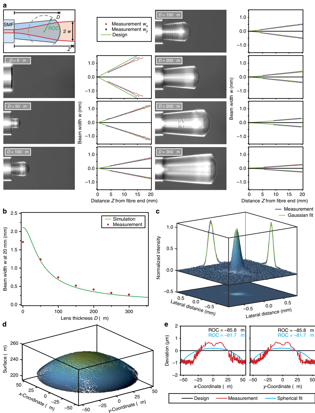
Figure 2 | Characterization of a spherical lens for the collimation of a Gaussian beam. (a) Optical microscope images of different spherical lenses with different thicknesses D ranging from 0 to 300 \mu m and the corresponding propagation measurements and simulations of the beam width w (radius of intensity at 1/e^2 ). The radius of curvatures are -25.6 , -38.1 , -53.5 , -69.5 , -85.8 and -102.1 \mu m for lens thicknesses D of 50, 100, 150, 200, 250 and 300 \mu m, respectively. (b) Beam width for each lens taken at a distance of 20 mm after the fibre end facet and the comparison with the simulation obtained by Gaussian beam propagation with an ABCD matrix formalism. (c) Intensity distribution of the beam profile at a distance of 10 mm measured from the optical fibre using a lens thickness D of 300 \mu m. (d) Measurement of the topography using optical interferometry of a spherical lens with a lens thickness D of 250 \mu m and a designed radius of curvature of -85.77 \mu m. (e) Deviation of the measured surface topography, which is well below 1 \mu m.
