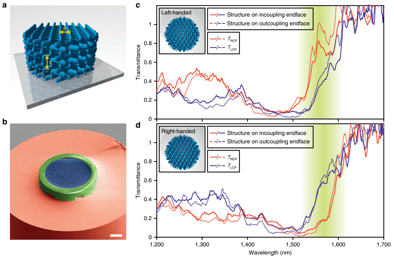
Figure 5 | Chiral photonic crystal structure for polarization control directly on an optical fibre tip. (a) Illustration of the ‘twisted woodpile’. (b) Coloured scanning electron microscope image of the fabricated left-handed structure (blue) containing a solid ring (green) in order to increase the stability and reduce deformation of the structure. (c,d) Measured transmittance spectra for right- and left-handed circularly polarized light for the chiral photonic crystal at the in-/out-coupling end facet of the optical fibre and for the left- and right-handed photonic crystal structure, respectively. The design wavelength for the polarization filter was 1,550 nm. Scale bar, 10 \mu\text{m} (b).
