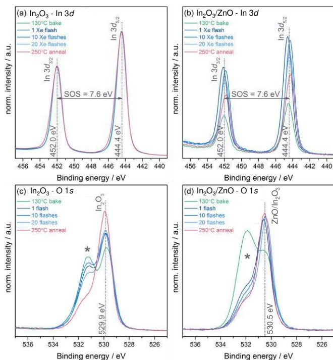
Fig. 5 In 3d and O 1s core level XPS spectra for (a) and (c) \text{In}_2\text{O}_3 layer, and (b) and (d) \text{In}_2\text{O}_3/\text{ZnO} heterostructure samples prepared using different methods, including photonic treatment and thermal annealing. A higher binding energy shoulder observed on the O 1s spectra is marked with an asterisk.
