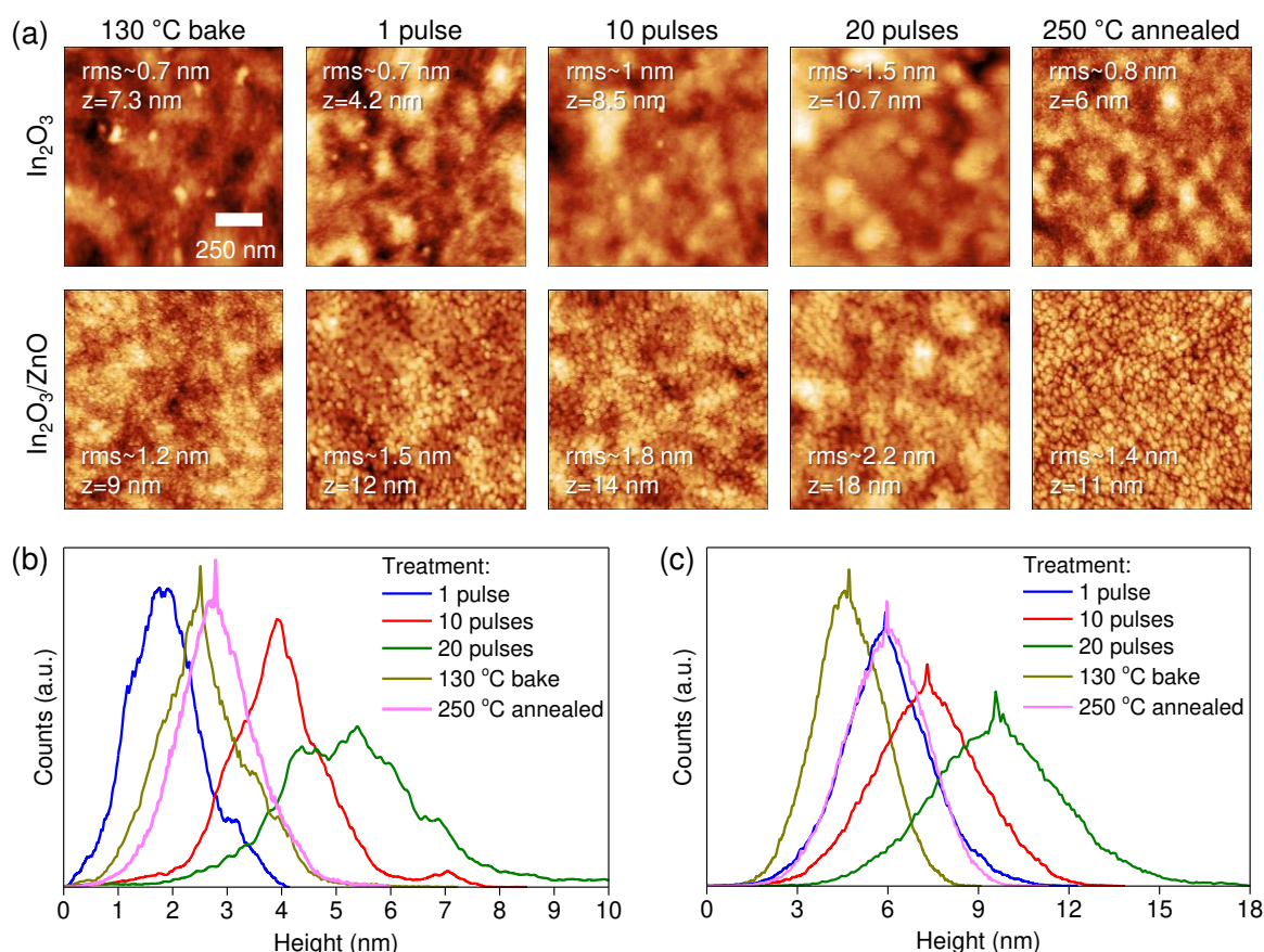
Fig. 4 (a) AFM surface topography images of \text{In}_2\text{O}_3 and \text{In}_2\text{O}_3/\text{ZnO} structures (deposited onto glass/ \text{Al}/\text{AlO}_x/\text{ZrO}_x structures) subjected to: low-temperature thermal annealing (bake), photonic treatment using varying number of pulses and conventional thermal annealing at 250 °C. Corresponding height distributions for (b) \text{In}_2\text{O}_3 and (c) \text{In}_2\text{O}_3/\text{ZnO} .
