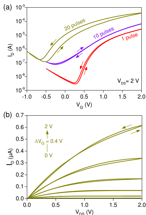
Fig. 2 (a) Transfer characteristics of heterostructure thin-film transistors consisting of photonicallly cured \text{In}_2\text{O}_3 films using 20 xenon pulses and single layer ZnO dried at 110^\circ\text{C} which were subsequently exposed to 1, 10 and 20 xenon flash pulses of energy densities of 5\text{ J/cm}^2 and pulse durations of 500\ \mu\text{s} at a fire rate of 1.2\text{ Hz} and (b) corresponding output characteristics for \text{In}_2\text{O}_3/\text{ZnO} transistors flashed each layer with 20 pulses.
