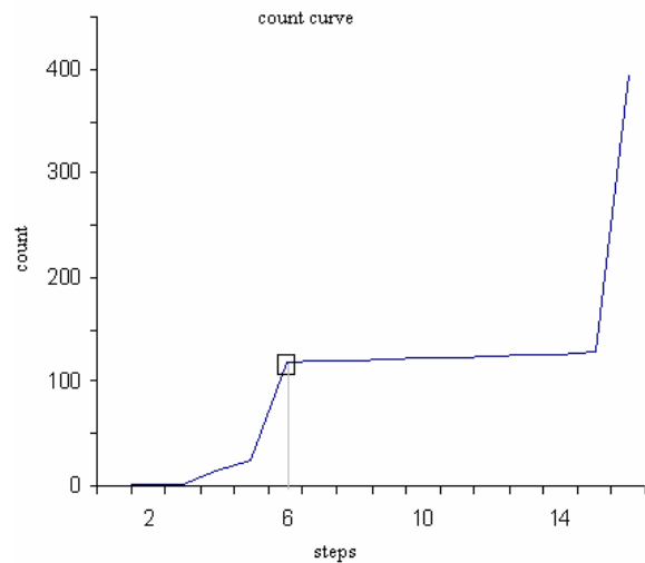
Figure 2. Count curve along a randomly chosen path through a subgoal state under the learned policy.
