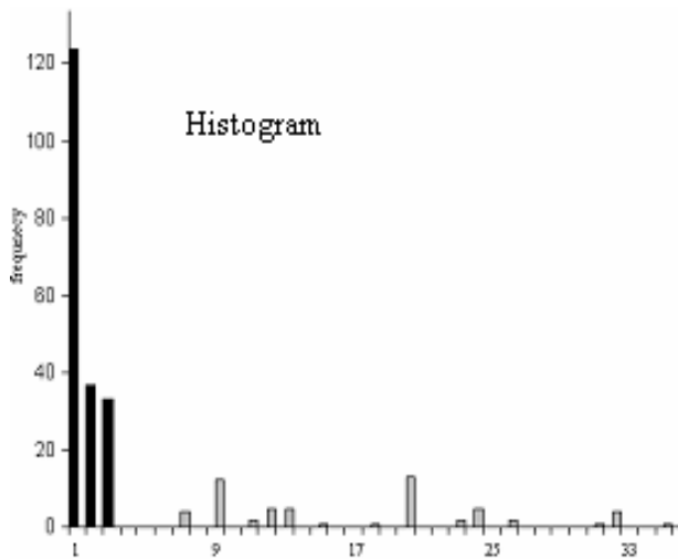
Figure 3. Histogram for the distribution of the gradient ratio in regular space (dark bars) and at subgoal states (light bars).
