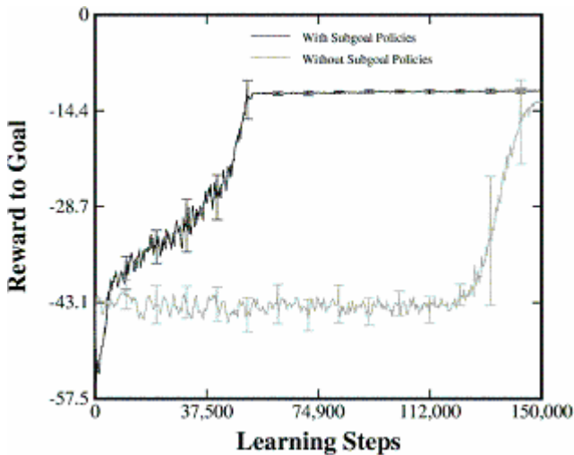
Figure 6. Comparison of learning speed using subgoal policies and using primitive actions only.
