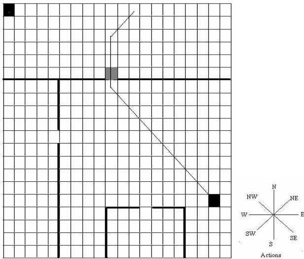
Figure 1. Set of primitive actions (right) and gridworld(left) with the initial state in the upper left corner, the goal in the lower right portion and a random path under the learned policy.
