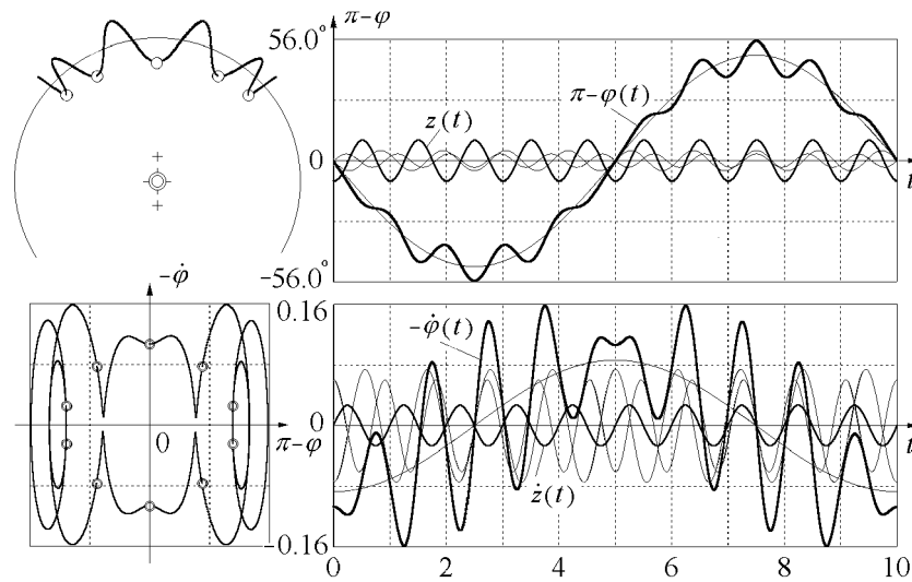
Figure 2. The spatial path, phase orbit with Poincaré sections and graphs of stationary period-10 oscillations. The graphs are obtained by a numerical integration of the exact differential equation (5) with \omega_0 = 0 and \gamma = 0 , for the momentary angular deflection \varphi(t) . Thin lines show separate harmonics. The fundamental harmonic with the frequency \omega/10 dominates the spectrum. The 9th and 11th harmonics have nearly equal amplitudes. Graphs of the axis motion z(t) and \dot{z}(t) are also shown.
