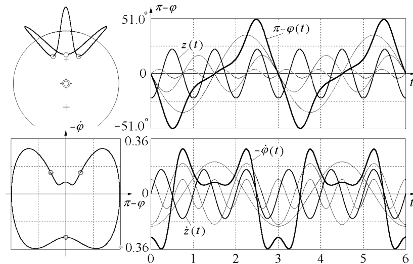
(no friction, no gravity, axis amplitude 0.45, initial defl. 180.0 degr., init. ang. velocity 0.2818)
