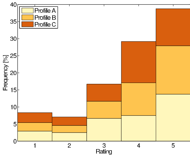
Fig. 3. Ratings distribution.
