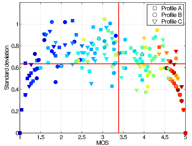
Fig. 5. Standard deviation of subjective ratings versus MOS. The red lines represent the respective medians. Points are colored according to the bit rate of the corresponding compressed HDR image.
